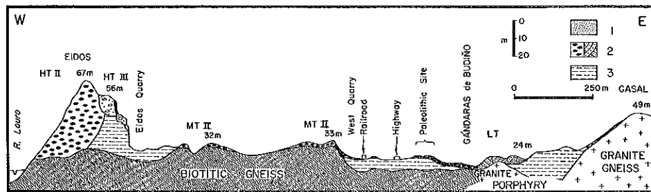
Fig. 2. Section of middle Louro Valley at the Budiño Site (Km 20 of the Vigo-Túy highway). 1 = Late Pleistocene colluvium; 2 = High (HT), Middle (MT) and Low (LT) gravel terraces of early to late Pleistocene; 3 = Mio-Pliocene kaolin and grit beds. All diagrams after detailed hand-level transects or line-level sections.
