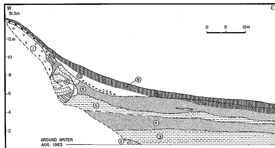
Fig. 7. North face of West Quarry (200 m west of Budiño Site). Symbols identified in text and Table 3. Patterns identical to those of Fig. 3.
