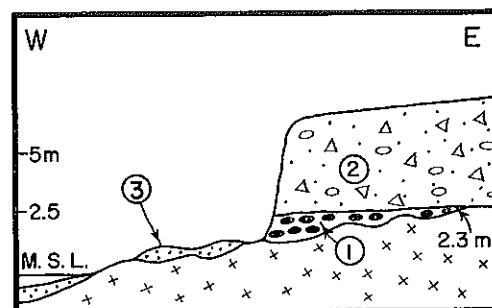
Fig. 10. Littoral and fluvial deposits at Playa de Patos. 1 = Last Interglacial (?) beach gravel; 2 = Late Pleistocene colluvium; 3 = modern beach sand.
