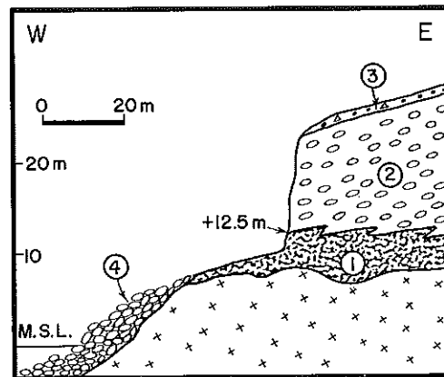
Fig. 12. Littoral and fluvial deposits at Sanjián, near Km 77.6. 1 = Detrital peat with date 28,400 B.P. (I-2261); 2 = Late Würm cobble gravels of Rio Cobo fan; 3 = humic, gritty colluvium; 4 = modern beach cobbles.
