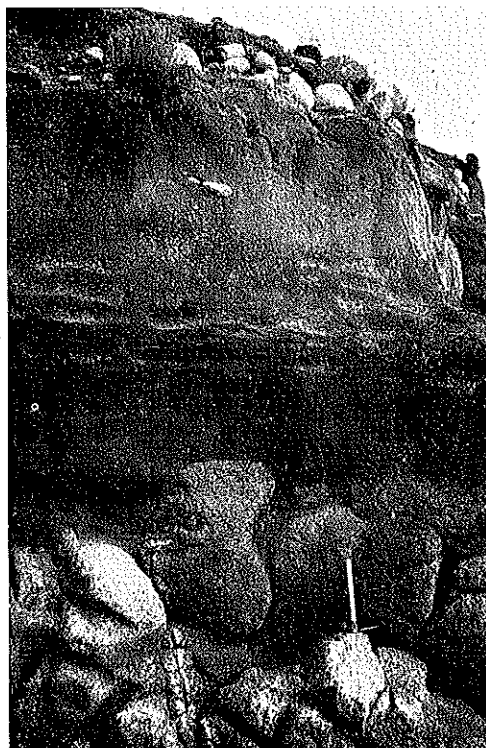
Fig. 11. Early Würm beds overlying wave-worn granite gneiss with Karrenkarst phenomena at Mougás (North) near Km 67.3. Sample I-2177 ("greater than 39,900 years") from black stratum of detrital organic matter, giving way at top to mineral deposits. Beach cobbles at top form part of artificial embankment and rest on A-horizon of recent soil.
