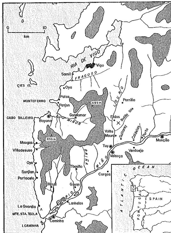
Fig. 1. The Vigo-Tuy area of Southwestern Pontevedra Province. Elevations above 400 meters shaded.
