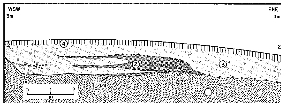
Fig. 4. Section of Trench C-IX P (Locality 2). 1 = Tertiary detrital Kaolin; 2 = Lower Colluvium, with grit-gravel (dark) and sandy (light) facies; 3 = Upper Colluvium (bed 6c of text); 4 = A-horizon of Holocene soil. I-2174 and I-2175 localize hearths from which radiocarbon samples were extracted.
