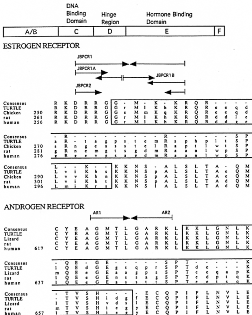
Fig. 8. Schematic of turtle estrogen receptor (ER) and androgen receptor (AR) gene. Top portion shows functional domains of steroid hormone receptors with subclones indicating regions sequenced below. The lower portion presents consensus sequence showing a portion of the deduced amino acid sequence for the turtle ER and AR and corresponding regions of published sequences for these hormone receptors of other species. Boxed segment of the sequence signifies the hinge region. Dashes in the consensus sequence indicate non-conserved amino acids.
