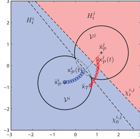
Fig. 2. If \mathbf{x}_{\mathcal{P}}^i \xrightarrow{0} \mathbf{x}_{\mathcal{T}} and there exists t > 0 such that \mathbf{x}_{\mathcal{T}}(t) \in \text{int } \mathcal{V}^j \cap H_t^j(\mathbf{x}_{\mathcal{P}}^i(t), \mathbf{x}_{\mathcal{P}}^j(t)) , where \mathbf{x}_{\mathcal{P}}^j(t) = \bar{\mathbf{x}}_{\mathcal{P}}^j , then the j^{\text{th}} pursuer will capture the target faster than T(t, \mathbf{y}^i(t); i) . As a result, the pursuer-target assignment is updated at t so that \mathbf{x}_{\mathcal{P}}^j \xrightarrow{t} \mathbf{x}_{\mathcal{T}} .
