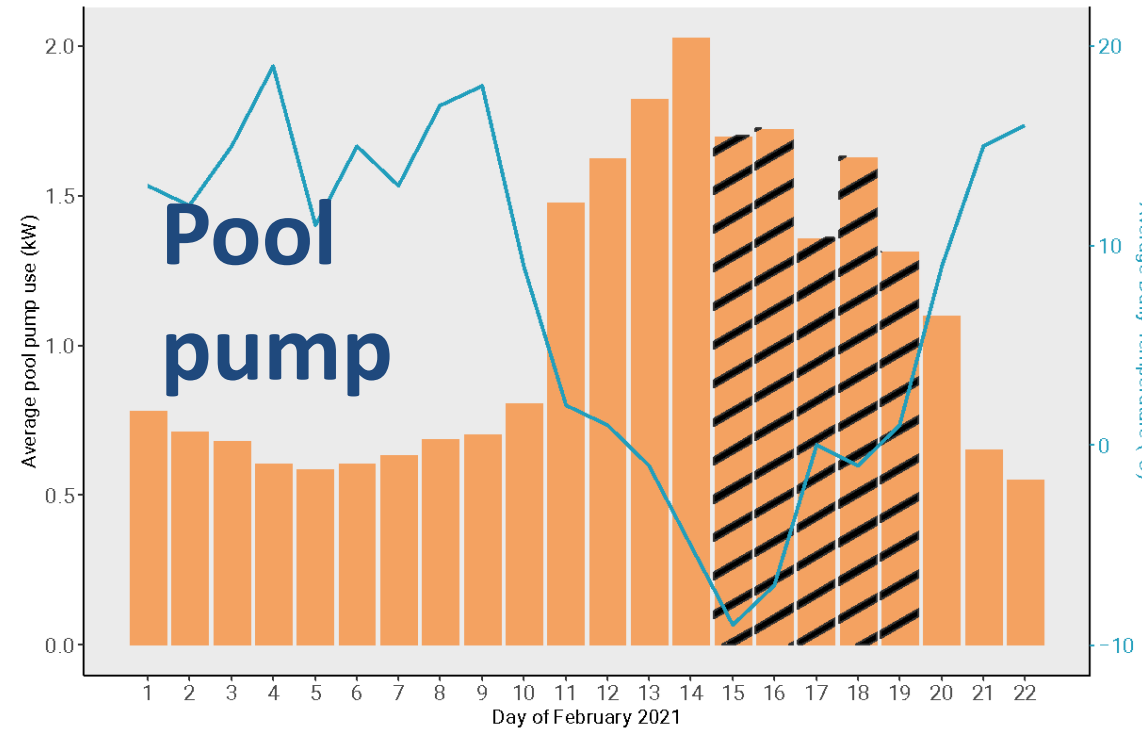
Average Home Daily Pool Pump Power Draw in February 2021 (kW)
