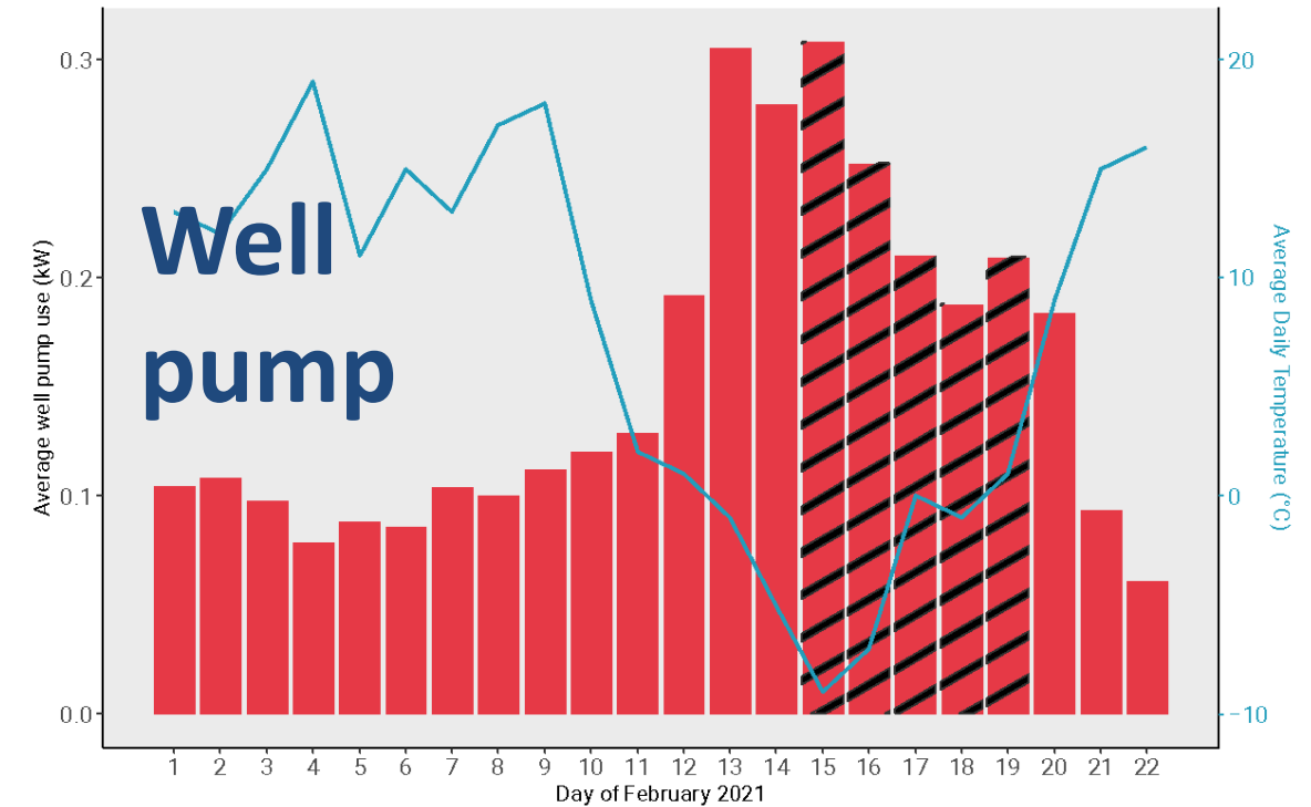
Average Home Daily Well Pump Power Draw in February 2021 (kW)
