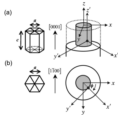
FIG. 3. (a) Cutaway and (b) cross-sectional diagrams of the coaxial nanostructure and corresponding orientation of the wurtzite crystal geometry. \{x, y, z\} denote the reference axes of the system while \{x', y', z'\} denote the normal, tangential, and longitudinal axes for a specific point on the circular interface corresponding to the angle \phi .
