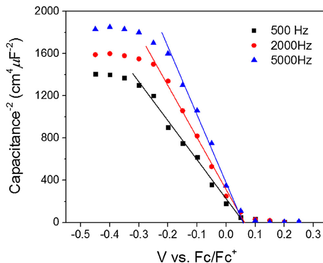
Fig. 4. Mott-Schottky plot of p- \text{MASnI}_3 in \text{CH}_2\text{Cl}_2 containing 0.1 M TBAPF 6 supporting electrolyte at 500 Hz, 2000 Hz, and 5000 Hz. The solid lines are linear fits to the experimental data.
