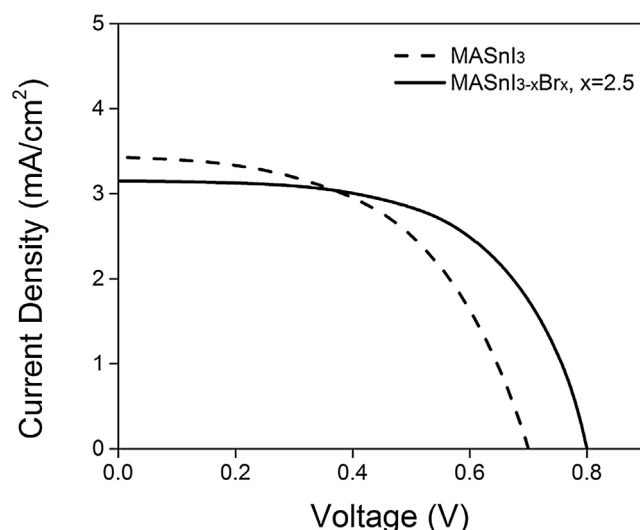
Fig. 6. Steady-state current density–voltage relation for p- \text{MASnI}_{0.5}\text{Br}_{2.5}/\text{CH}_2\text{Cl}_2 , BQ (2 mM), BQ •- (2 mM)/C and p- \text{MASnI}_3/\text{CH}_2\text{Cl}_2 , BQ (2 mM), BQ •- (2 mM)/C PEC solar cells under irradiation with a 100 mW/cm 2 xenon lamp focused onto the photoelectrode. The optical path through the solution was about 0.3 mm.
