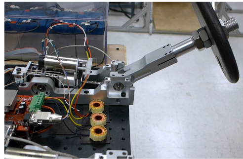
b) High-power test upper position
