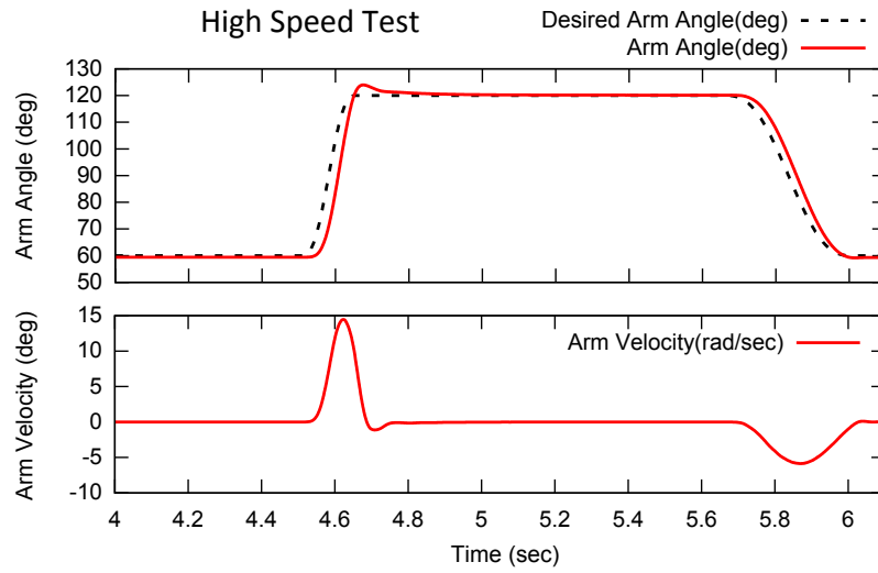
Figure 4.10: High-speed position tracking test. The actuator output follows a reference signal that changes 60 degrees in less than 0.2 seconds. The actuator is able to track the reference signal closely and reaches the maximum mechanical speed of the ball screw of 15 rad/sec. The torque moment arm ( L ) rotates through its largest length at \theta_a = 90^\circ .
