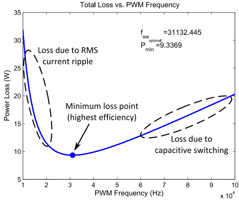
Figure 3.12: Optimization of PWM frequency for minimum loss in electric motor drives. Using (3.8) we can find the optimal PWM frequency which minimizes loss between the switching elements in the servo drive and current ripple in the electric motor.
