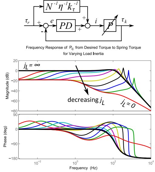
b) Closed-loop frequency response with variable SEA inertia
