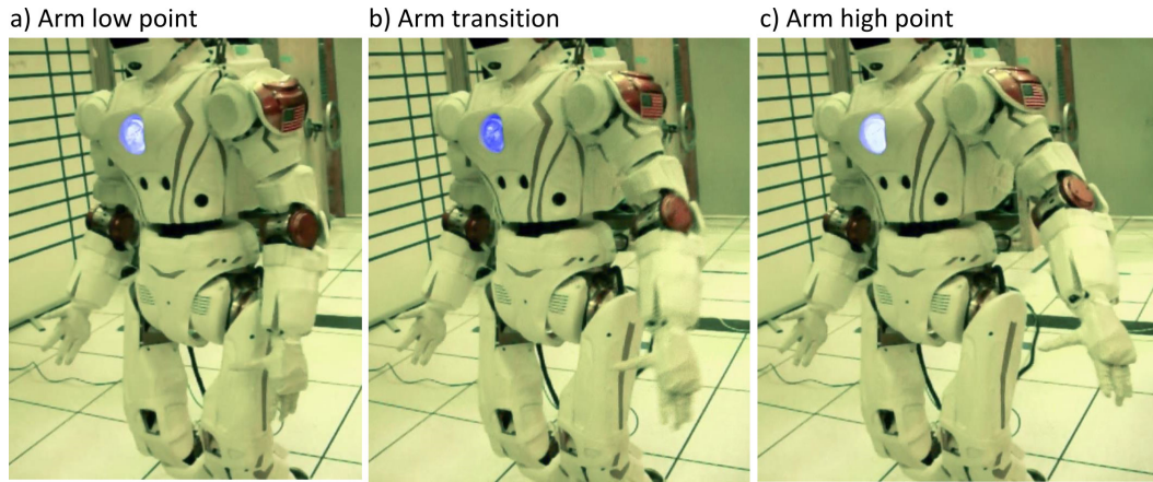
Figure 6.11: Experiment 2: Coordinated Motion. Valkyrie arm joints J1 through J4 are placed in torque control mode and are supplied desired torque signals according to the controller shown in Figure 6.10. As a result, each joint roughly tracks a sinusoidal position.
