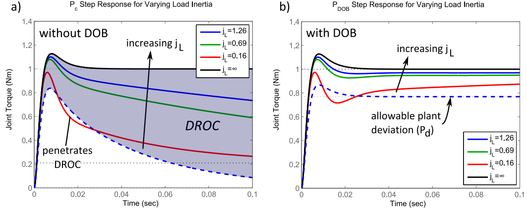
Figure 5.6: Time domain representations of Figures 5.5a and 5.5b. In a) the step response of only the inner portion of the proposed force controller ( P_c ) to various load inertias is shown. Again, for these control parameters, all values of load inertia except j_L = 0.16 \text{ Kg} \cdot \text{m}^2 remain within the DROC. In b) step responses are shown for the same SEA plant parameters as in a) , but a DOB is now applied. The DOB is shown to dramatically improve low-frequency performance, maintaining both Valkyrie inertia values within the allowable performance envelope.
