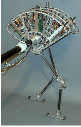
a) Spring Flamingo and its SEA
