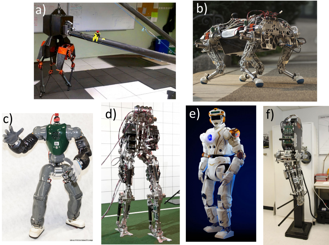
Figure 1.6: A few examples of high-performing robots with series elastic actuators: a) Atrias 2.1 9 (Hereid et al., 2014), b) StarLETH 10 (Hutter, 2013), c) Coman 11 (Li et al., 2012), d) Saffir 12 (Lee et al., 2013), e) Valkyrie 13 (NASA-JSC, 2013), and f) Hume 14 (Slovich et al., 2012).
