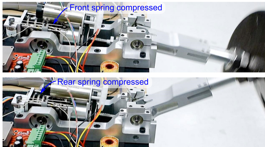
c) Actuator dynamics during test
