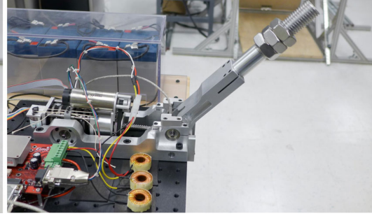
Figure 4.9: High-speed position tracking test setup.
