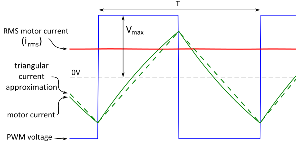
Figure 3.6: Current waveform induced by a PWM voltage applied to a motor.
