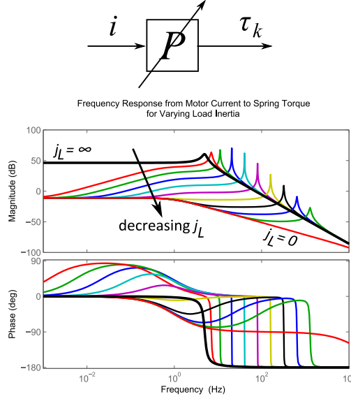
Figure 5.2: a) Series of SEA control plants (5.6) for varying load inertia. Reducing load inertia is shown to increase resonant frequency and alter effective level of damping in the response. b) Closed-loop ( P_c in Figure 4.3c) torque response for a series of SEA plants with decreasing j_L . For larger values of j_L , the bandwidth of the system remains fairly constant while only low frequency behavior changes.
