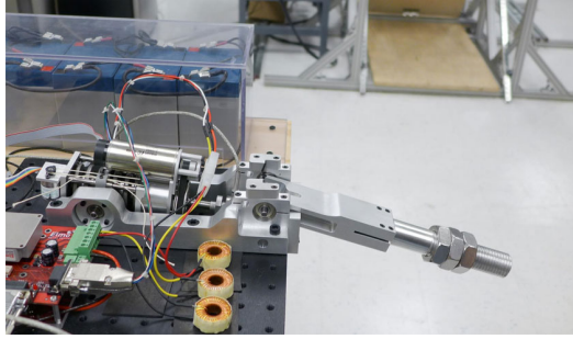
Figure 4.9: High-speed position tracking test setup.
