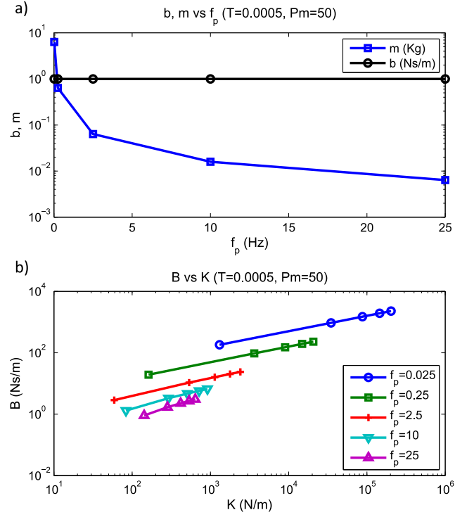
Figure 7.9: a) Search space of m and b for the experiment shown in Figure 7.8. b) Solution space of K and B for the experiment shown in Figure 7.8. Each point represents a K , B pair producing a system with the target phase margin.
