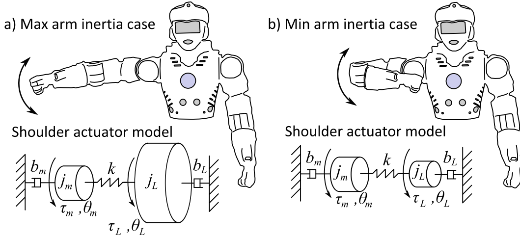
Figure 5.1: An example of a variable load inertia scenario using the abduction/adduction shoulder joint of NASA-JSC’s Valkyrie robot. Approximate actuator-level models are shown for each case, a large load inertia corresponding to the outstretched case and a smaller load inertia corresponding to the bent-elbow case.
