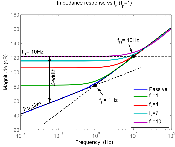
Figure 7.7: Impedance frequency response ( F_{ext}/X ) of an actuator with various closed-loop gains ( K, B, \zeta_d = 1 ) determined by f_n . With K and B set to zero, the impedance response is that of the passive actuator. The open loop passive corner frequency ( f_p ) is shown as well as the closed-loop natural frequency ( f_n ) for f_n = 10\text{Hz} . The difference between maximum and passive impedance, Z-width, is also illustrated.
