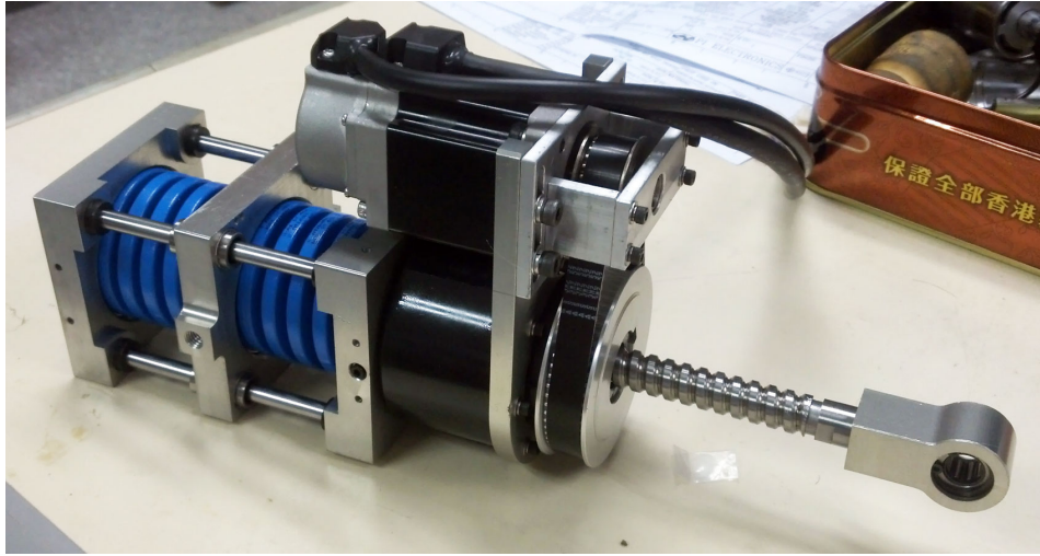
Figure 2.14: Stone Age Robotics SEA based on UT-SEA design.
