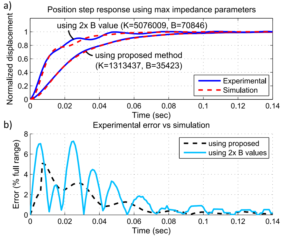
Figure 7.15: Full Actuator Experiment. The same experiment was performed as was described in Figure 7.14 except with the full actuator. While the experimental data closely matches simulation data, larger discrepancies can be seen compared to Figure 7.14. The cause of this increase is likely due to the drivetrain dynamics (particularly the belt). As was the case in the motor experiment, our method again correctly chooses the maximum critically damped control parameters with a phase margin of 50 degrees. The step displacement for this test was 2mm. Due to the high gains used, a higher displacement would cause current saturation to occur (30 amp limit).
