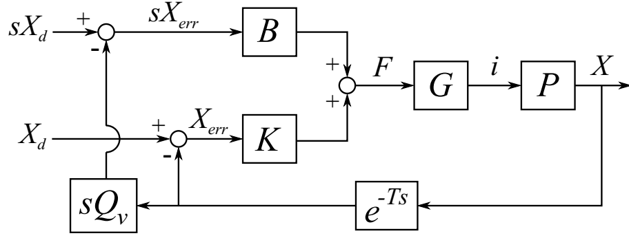
Figure 7.2: A spring-damper ( K - B ) impedance control model with delay ( e^{-Ts} ) and velocity filtering ( Q_v ). No force feedback is used, desired forces are simply translated into desired currents.
