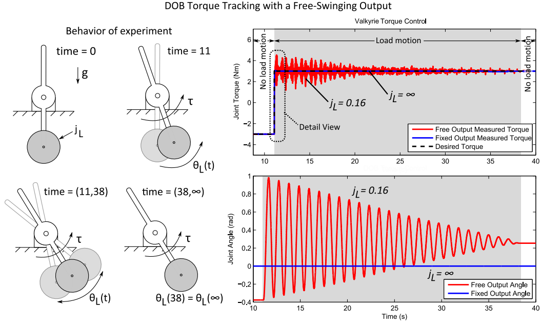
Figure 5.9: Step response of the DOB torque controller used on Valkyrie (Figure 4.3c) to a torque command for two different load inertias. Due to the low friction of the DOB-based controller, the torque step induces high velocity pendular swinging at the actuator output that persists for almost 30 seconds. See Figure 5.10 for a detailed view of the torque response.
