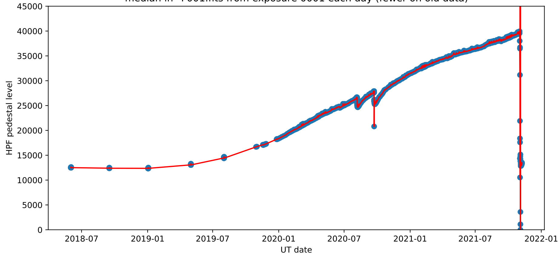
median in *F001.fits from exposure 0001 each day (fewer on old data)
