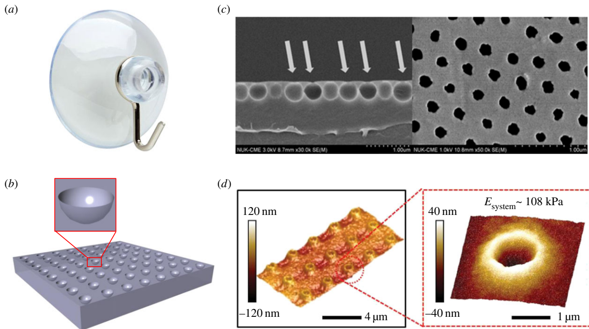
Figure 1. (a) A thin-walled suction cup fixture. (b) A 3D schematic of a crated surface. (c) SEM images of closely packed sub-micron-sized surface dimples on UV resin (adopted from Chang et al. [2] with permission from Copyright (2017) American Chemical Society). (d) AFM images of 1\ \mu\text{m} diameter craters on the surface of polydimethylsiloxane (PDMS) (adopted from Choi et al. [6] with permission from Copyright Wiley-VCH Verlag GmbH & Co. KGaA).
