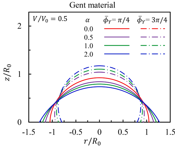
Fig. C1. Profiles of droplets confined by Gent membranes subjected to sliding boundary conditions. V/V_0 = 0.5 is prescribed while the elastocapillary number \alpha is varying. Solid curves correspond to \bar{\phi}_Y = \pi/4 and dash-dot curves for \bar{\phi}_Y = 3\pi/4 . The two red curves overlay.
