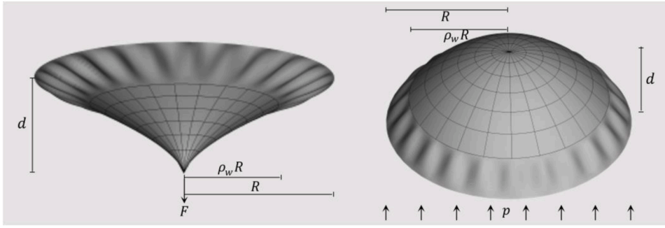
Fig. 8. Schematics of exploiting the wrinkling instabilities in the suspended region in indentation and bulge tests of thin sheets.
