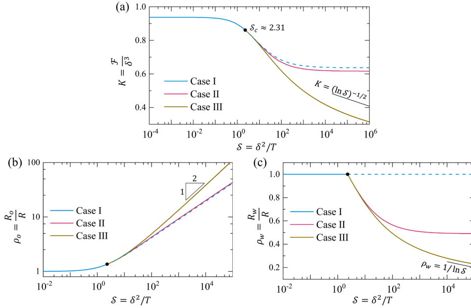
Fig. 6. The dependency of the effective stiffness (a), the sliding extent (b), and the wrinkling extent (c) on the sliding number in all three cases. Dots label the critical points from Case I to Case II (strong adhesion) or to Case III (weak adhesion). Dashed curves represent unrealistic Case I solutions after instability sets in.
