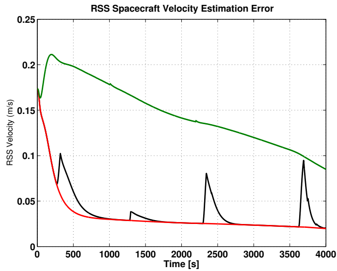
Figure 9 Comparison of velocity estimation error, green line shows no threshold, black line with threshold and red line is the new algorithm
