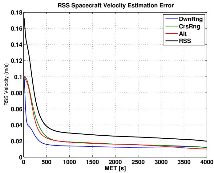
Figure 7. Velocity Estimation Error New Algorithm
