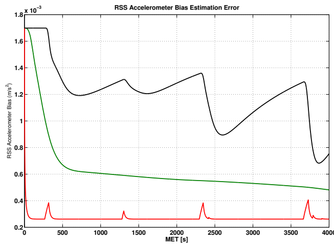
Figure 10 Comparison of accelerometer bias estimation error, green line shows no threshold, black line with threshold and red line is the new algorithm
