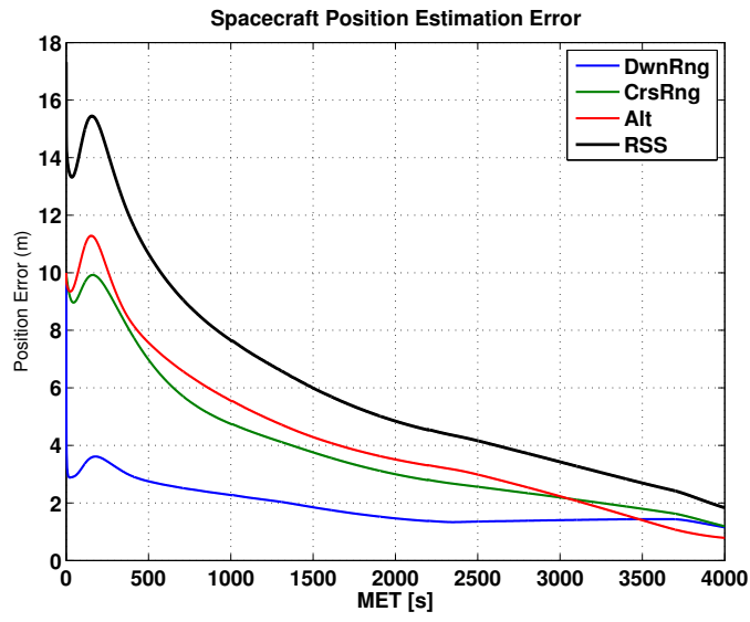
Figure 6. Position Estimation Error New Algorithm
