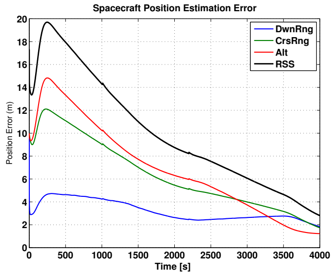
Figure 2. Position Estimation Error Without Thresholding
