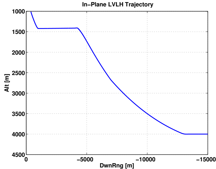
Figure 1. Relative In-Plane LVLH Trajectory
