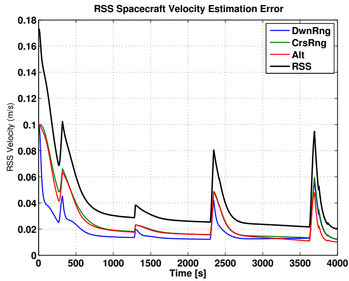
Figure 5. Velocity Estimation Error With Thresholding
