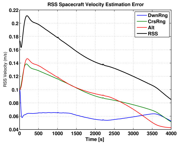
Figure 3. Velocity Estimation Error Without Thresholding
