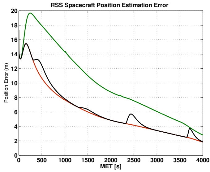
Figure 8 Comparison of position estimation error, green line shows no threshold, black line with threshold and red line is the new algorithm
