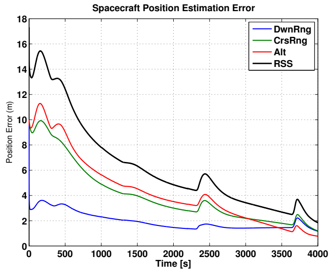
Figure 4. Position Estimation Error With Thresholding
