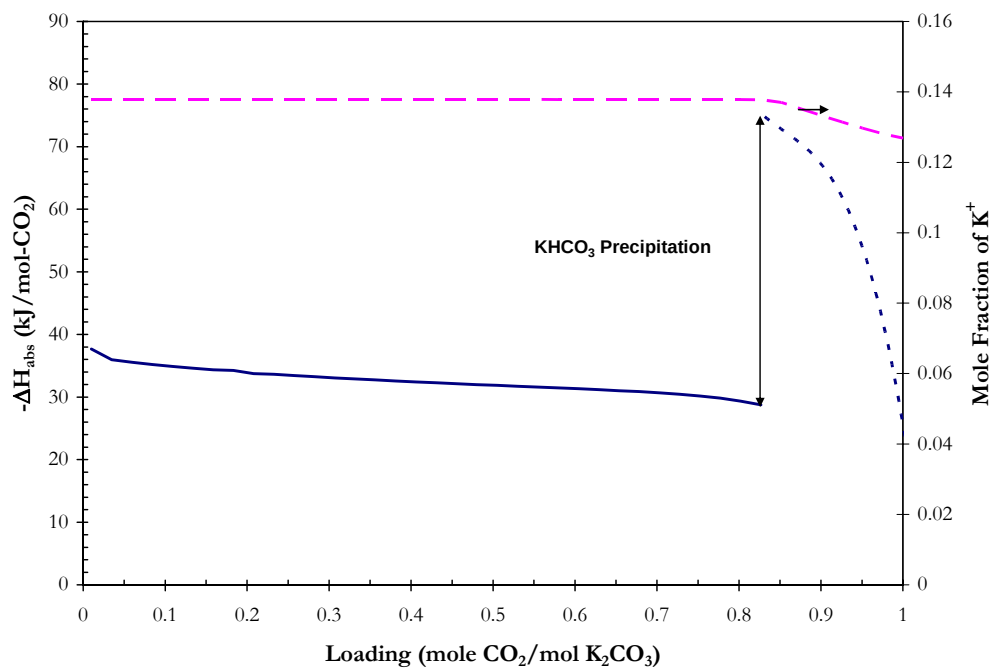
Figure 12.8-32. Predictions for the Differential Enthalpy of CO 2 Absorption from the elecNRTL Model in 40 wt % K 2 CO 3 solutions at 90 °C.
