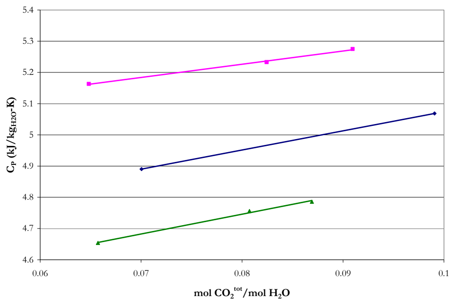
Figure 15.5-38. Apparent Partial Specific Heat Capacity for Mixtures of Potassium Carbonate + Piperazine at 40 °C. Points: \blacklozenge , 5 m K + + 2.5 m PZ, \blacksquare , 3.6 m K + + 3.6 m PZ, \blacktriangle , 6 m K + + 1.2 m PZ. Lines: OLS Approximations.
