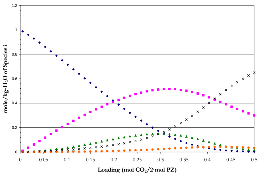
Figure 14.5-43. Predictions for the Liquid Phase Speciation in 1.0 m PZ at 25 °C from this work. Points: \blacklozenge , PZ, \blacksquare , PZH + , \blacktriangle , PZCOO -1 , \bullet , PZ(COO -1 ) 2 , \times , H + PZCOO -1 .
