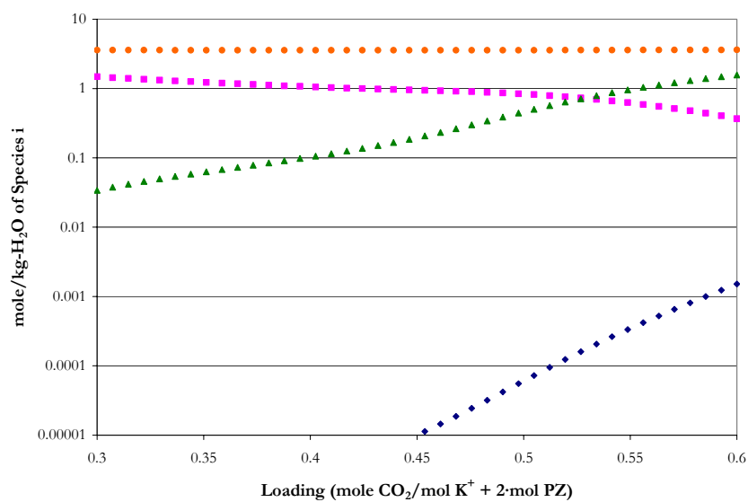
Figure 15.5-108. Predictions for the Liquid Phase Speciation in 3.6 m K + + 1.8 m PZ at 40 °C from this work. Points: ◆, CO 2 , ■, CO 3 -2 , ▲, HCO 3 - , ●, K + .
