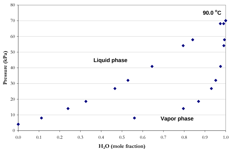
Figure 8.2-4. Isothermal VLE at 90.0 °C. Points: ♦, Tochigi et al. (1999).
