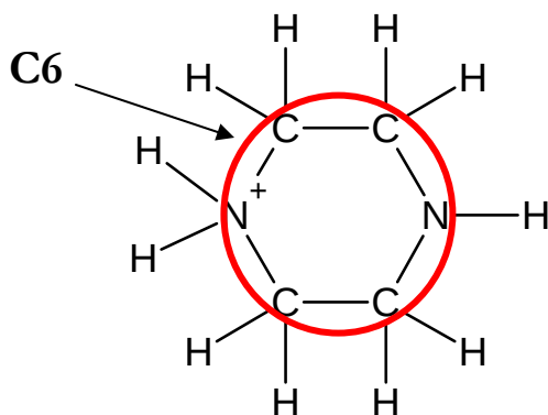
Figure 3.5-6 Molecular structure and active nuclei of carbons associated with PZ and PZH + .
