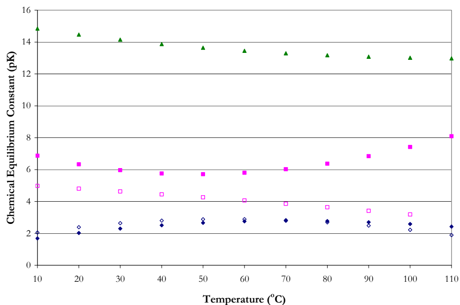
Figure 15.5-122. Comparison of the MEA and PZ Carbamate and Bicarbonate Based Chemical Equilibrium Constants from this work. Points: PZCOO -1 : \blacklozenge , this work, \diamond , Chapter XIV, PZ(COO -1 ) 2 : \blacksquare , this work, \square , Chapter XIV, MEACOO -1 : \blacktriangle , Chapter XIII.
