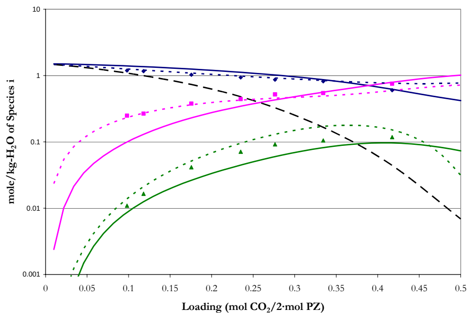
Figure 14.5-62. Comparison of Liquid Phase NMR Speciation in 1.5 m PZ at 40 °C to Model Predictions. Points: \blacklozenge , \text{PZ} + \text{PZH}^{+1} , \blacksquare , \text{PZCOO}^{-1} + \text{H} + \text{PZCOO}^{-1} , \blacktriangle , \text{PZ}(\text{COO}^{-1})_2 from Ermatchkov et al. (2003). Lines: - - -, Hilliard (2005), —, this work, — —, Conc. Free PZ.
