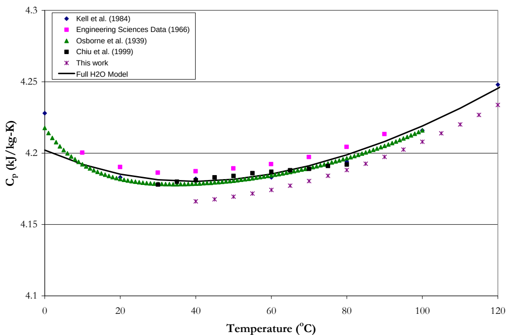
Figure 7.4-5. Expansion of Figure 7.4-3 from 0 – 120 ^{\circ} C for the Comparison of Model Predictions with Experimental Data for the Specific Heat Capacity of H 2 O.
