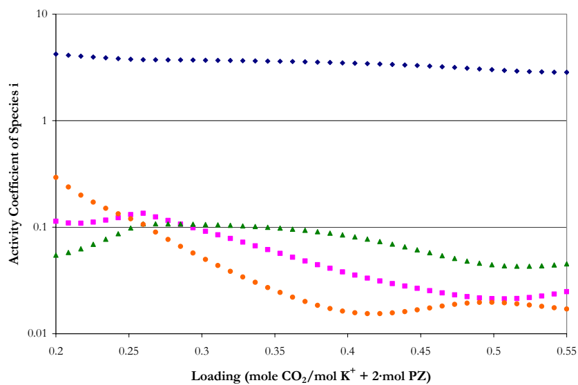
Figure 15.5-60. Predictions for the Liquid Phase Activity Coefficients in 3.6 m K^+ + 3.6 m PZ at 27 °C from this work. Points: \blacklozenge , CO_2 , \blacksquare , CO_3^{-2} , \blacktriangle , HCO_3^{-1} , \bullet , K^+ .
