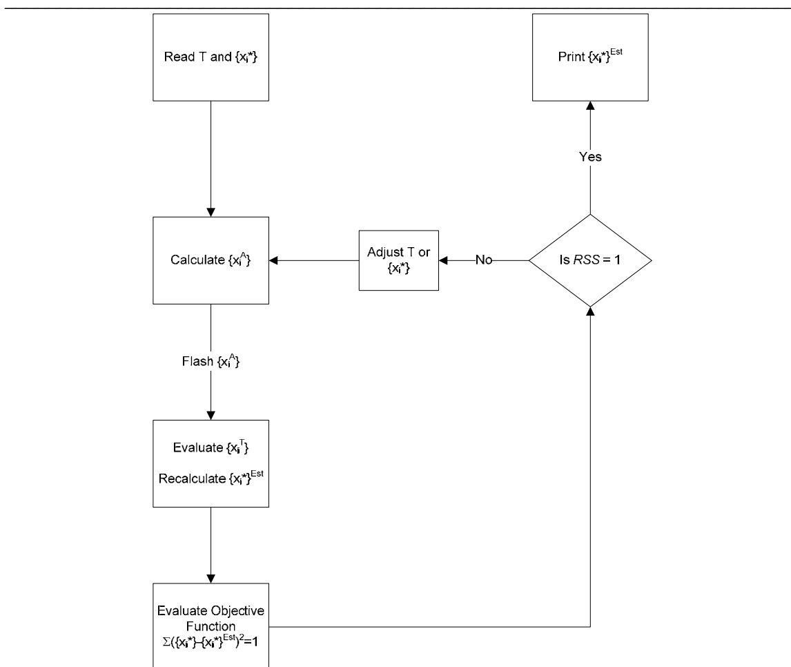
Figure 13.3-13. NMR Speciation Fortran Subroutine Schema Developed for Aspen Plus™.
