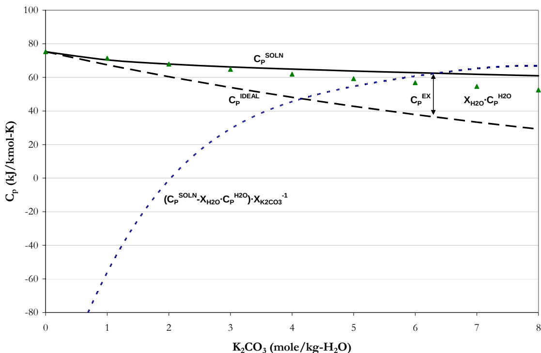
Figure 12.8-7. Comparison of the Molar Heat Capacity Predictions for H_2O - K_2CO_3 Mixtures at 40 °C from the elecNRTL Model to the Ideal Molar Heat Capacity based on the Constituent Components and Equation 12-41.
