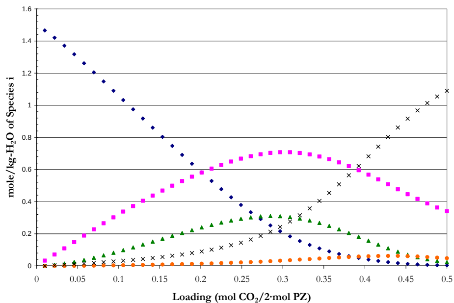
Figure 14.5-58. Predictions for the Liquid Phase Speciation in 1.5 m PZ at 25 °C from this work. Points: \blacklozenge , PZ, \blacksquare , PZH + 1, \blacktriangle , PZCOO - 1, \bullet , PZ(COO - ) 2 , \times , H + PZCOO - 1.
