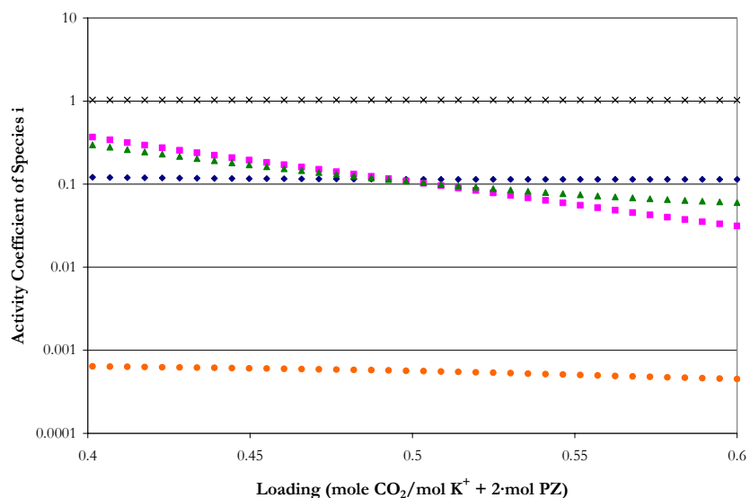
Figure 15.5-99. Predictions for the Liquid Phase Activity Coefficients in 3.6 m K^+ + 0.6 m PZ at 60 °C from this work. Points: \blacklozenge , PZ, \blacksquare , PZH^{+1} , \blacktriangle , PZCOO^{-1} , \bullet , PZ(COO^{-1})_2 , \times , H^+PZCOO^{-1} .
