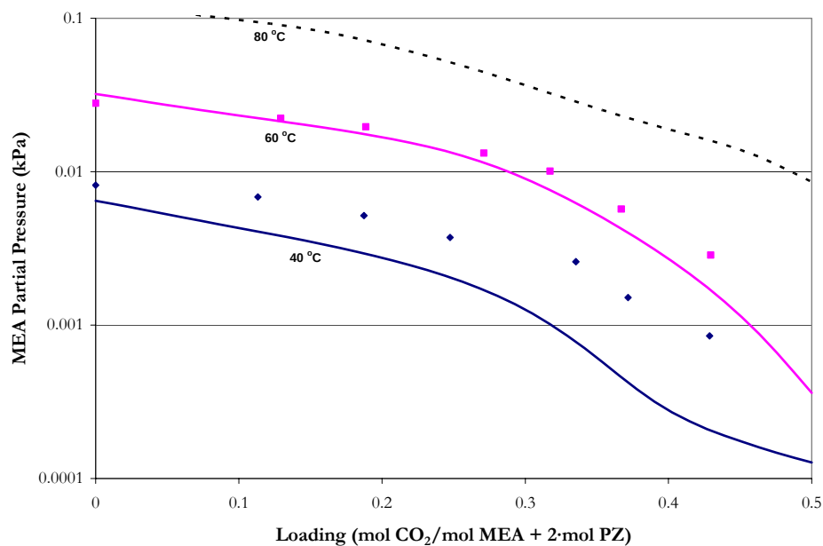
Figure 16.3-20. Experimental MEA Volatility in Mixtures of 7 m MEA Plus 3.6 m PZ from 40 to 80 °C from this work. Points: ♦ (40 °C) and ■ (60 °C). Lines: elecNRTL Predictions.
