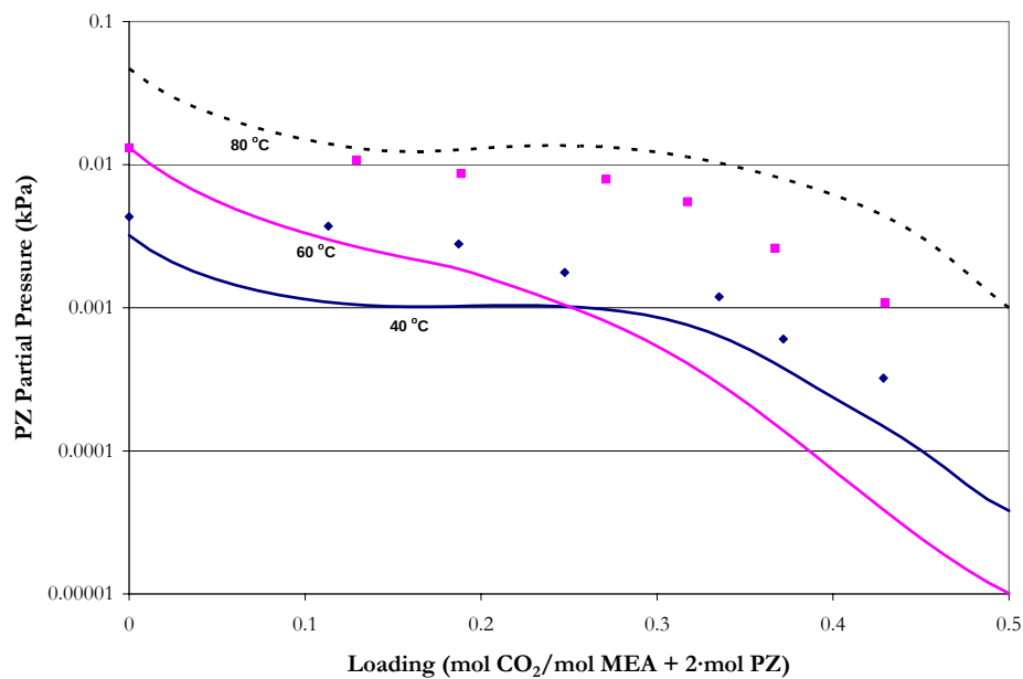
Figure 16.3-21. Experimental PZ Volatility in Mixtures of 7 m MEA Plus 3.6 m PZ from 40 to 80 °C from this work. Points: ♦ (40 °C) and ■ (60 °C). Lines: elecNRTL Predictions.
