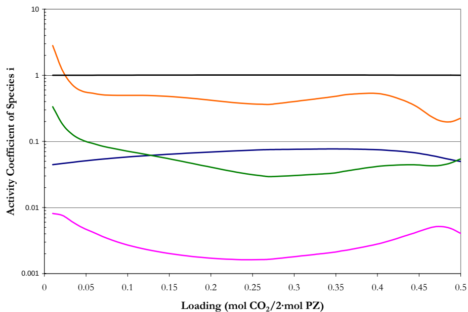
Figure 14.5-74. Predictions for the Liquid Phase Activity Coefficients in 5 m PZ at 40 °C from this work. Lines: —, PZ, —, PZH + 1, —, PZCOO - 1, —, PZ(COO - ) 2 , —, H + PZCOO - 1.
