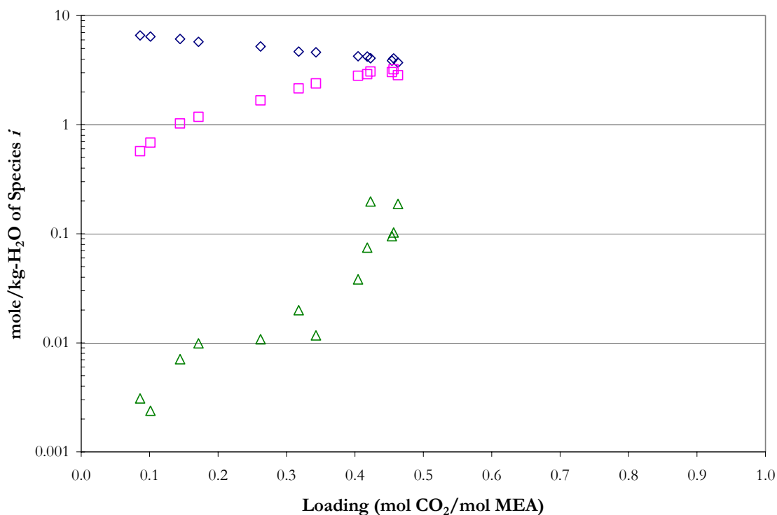
Figure 13.3-14. Liquid Phase Speciation from C 13 NMR at 27 °C. Points: \diamond , MEA+MEA + , \square , MEACOO - , \triangle , CO 3 -2 +HCO 3 -1 , from this work.
