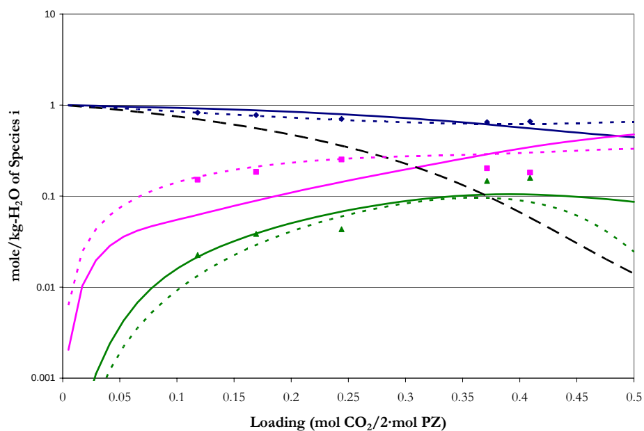
Figure 14.5-52. Comparison of Liquid Phase NMR Speciation in 1.0 m PZ at 60 °C to Model Predictions. Points: \blacklozenge , \text{PZ}+\text{PZH}^{+1} , \blacksquare , \text{PZCOO}^{-1}+\text{H}^{+}\text{PZCOO}^{-1} , \blacktriangle , \text{PZ}(\text{COO}^{-1})_2 from Ermatchkov et al. (2003). Lines: - - -, Hilliard (2005), —, this work, — —, Conc. Free PZ.
