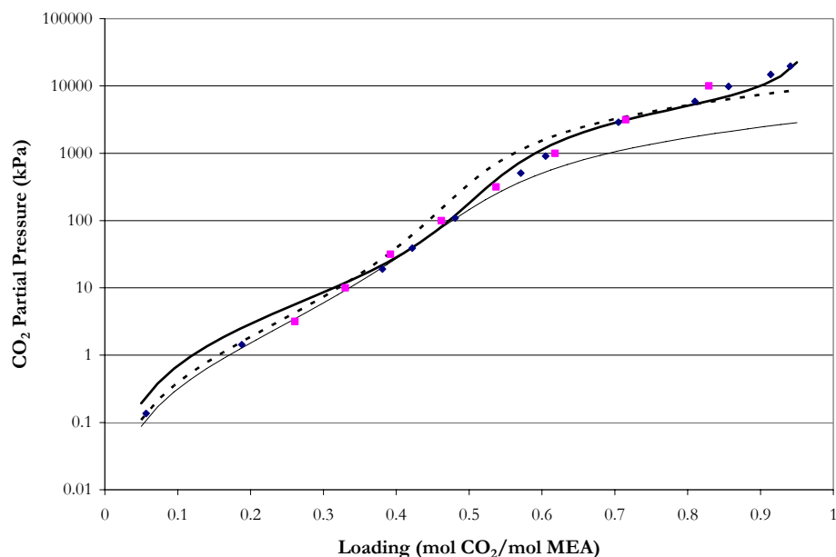
Figure 13.5-11. Comparison between Experimental and Predicted \text{CO}_2 Solubility in \sim 7 m MEA at 100^\circ\text{C} . Points: \blacksquare , Lee et al. (1976), \blacklozenge , Jou et al. (1995). Lines: \cdots , Austgen (1989), --- , Freguia (2002), — , this work.
