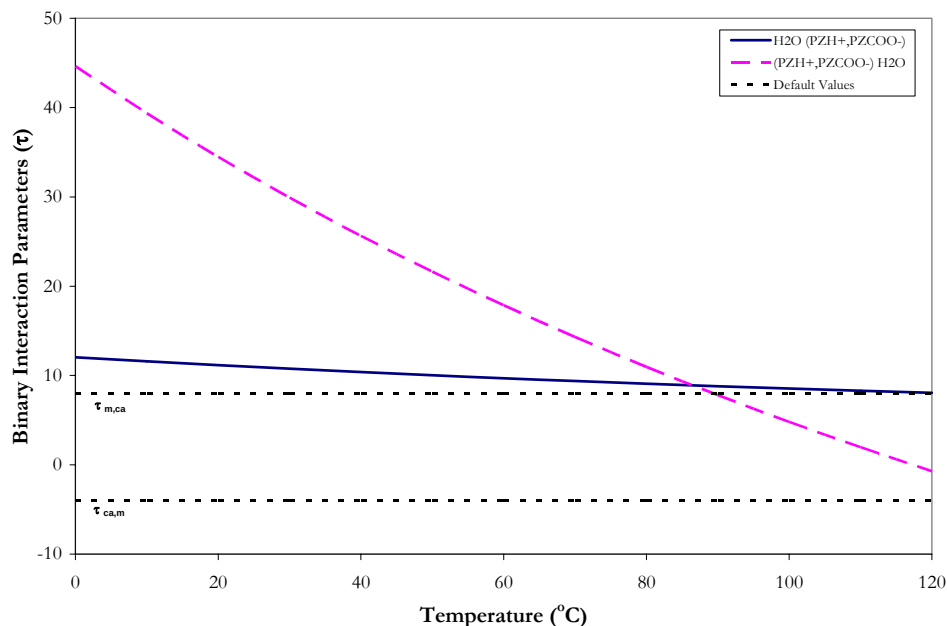
Figure 14.4-1. Binary Interaction Parameters for \text{H}_2\text{O} , \text{PZH}^{+1}/\text{PZCOO}^{-1} .
