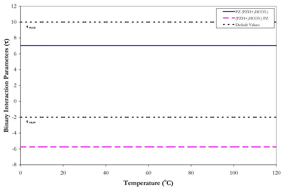
Figure 14.4-3. Binary Interaction Parameters for PZ, PZH + / HCO 3 - .
