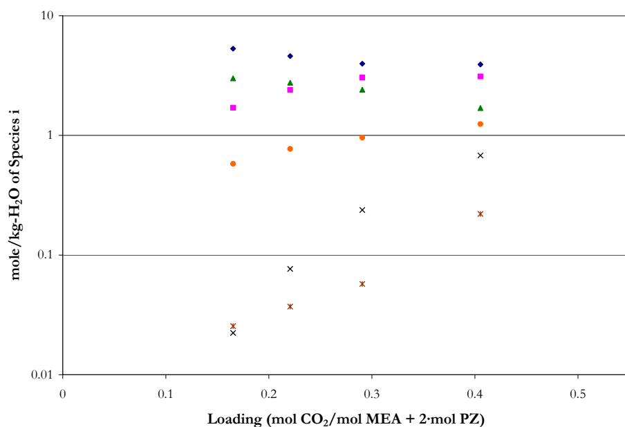
Figure 16.2-21. Liquid Phase Speciation from C 13 NMR at 40 °C. Points: ◆, MEA + MEAH + , ■, MEACOO - , ▲, PZ + PZH + , ●, H + PZCOO - + PZCOO - , ×, PZ(COO - ) 2 , *, CO 3 -2 +HCO 3 - .
