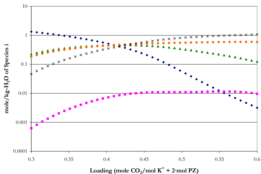
Figure 15.5-107. Predictions for the Liquid Phase Speciation in 3.6 m K + + 1.8 m PZ at 40 °C from this work. Points: ◆, PZ, ■, PZH + , ▲, PZCOO - , ●, PZ(COO - ) 2 , ×, H + PZCOO - .
