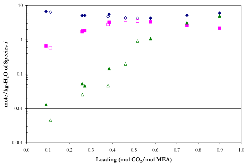
Figure 13.3-15. Liquid Phase Speciation from C 13 NMR at 40 °C. Points: ◆, MEA+MEA+H + , ■, MEACOO - , ▲, CO 2 +CO 3 -2 +HCO 3 -1 , from Poplsteinova (2004); ◇, MEA+MEA+H + , □, MEACOO - , △, CO 3 -2 +HCO 3 -1 , from this work.
