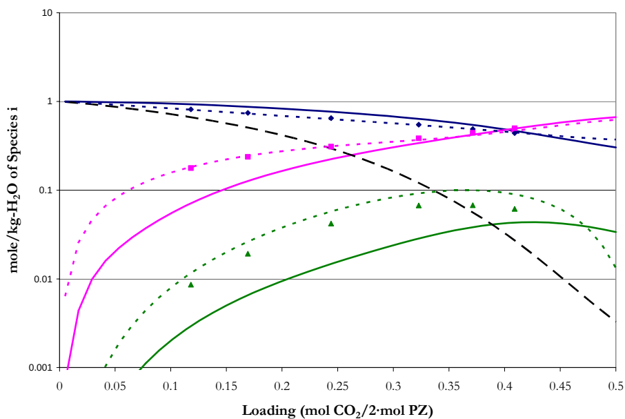
Figure 14.5-42. Comparison of Liquid Phase NMR Speciation in 1.0 m PZ at 25 °C to Model Predictions. Points: \blacklozenge , PZ+PZH + , \blacksquare , PZCOO -1 +H + PZCOO -1 , \blacktriangle , PZ(COO -1 ) 2 from Ermatchkov et al. (2003). Lines: ---, Hilliard (2005), —, this work, — —, Conc. Free PZ.
