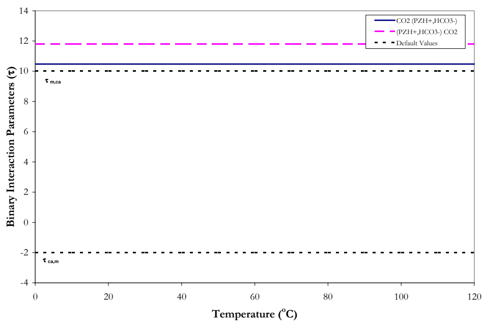
Figure 14.4-5. Binary Interaction Parameters for \text{CO}_2 , \text{PZH}^{+1}/\text{HCO}_3^{-1} .
