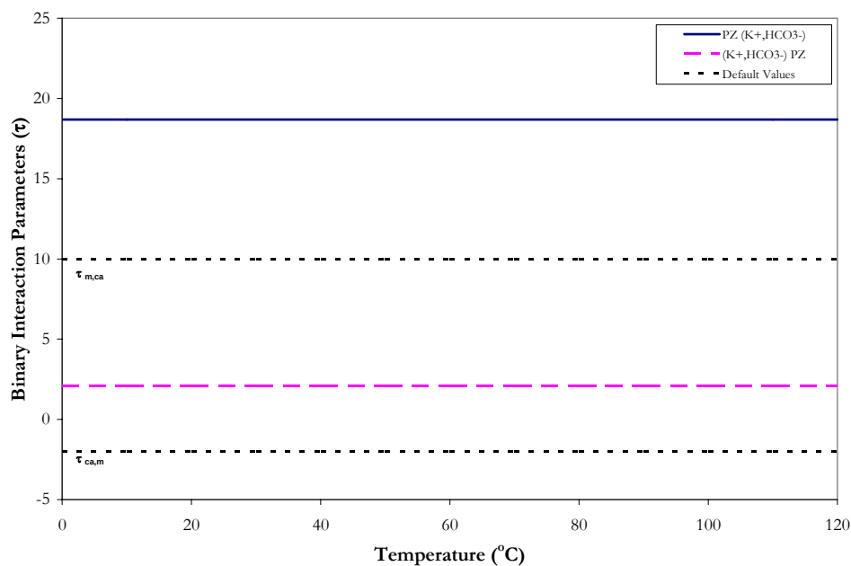
Figure 15.4-4. Binary Interaction Parameters for PZ, \text{K}^+/\text{HCO}_3^{-1} .
