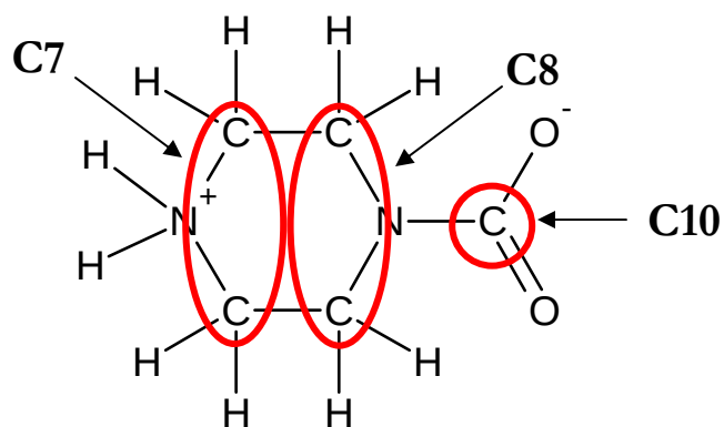
Figure 3.5-7 Molecular structure and active nuclei of carbons associated with PZCOO - and H + PZCOO -1 .
