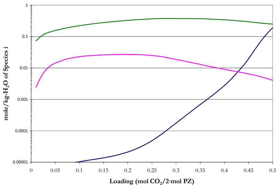
Figure 14.5-73. Predictions for the Liquid Phase Speciation in 5 m PZ at 40 °C from this work. Lines: —, CO 2 , —, CO 3 -2 , —, HCO 3 -1 .
