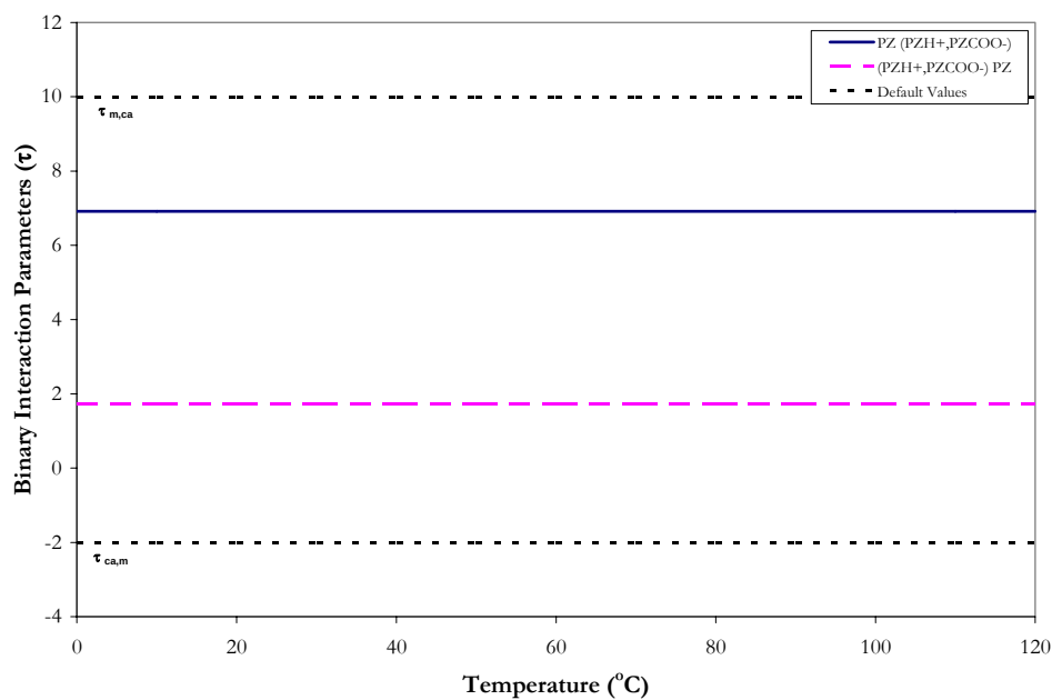
Figure 14.4-4. Binary Interaction Parameters for PZ, \text{PZH}^{+1}/\text{PZCOO}^{-1} .
