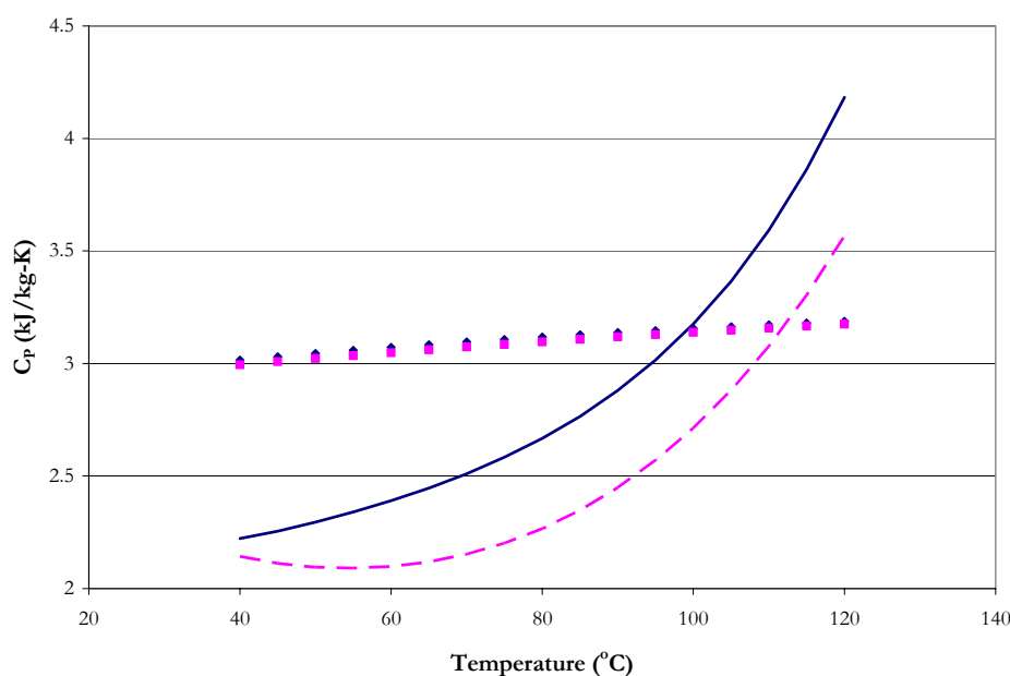
Figure 15.5-31. Comparison of Experimental Specific Heat Capacity in Loaded 5 m K + + 2.5 m PZ Mixtures from 40 to 120 °C. Points: ◆, Ldg = 0.39, ■, Ldg = 0.55. Lines: —, Ldg = 0.39, - - -, Ldg = 0.55.
