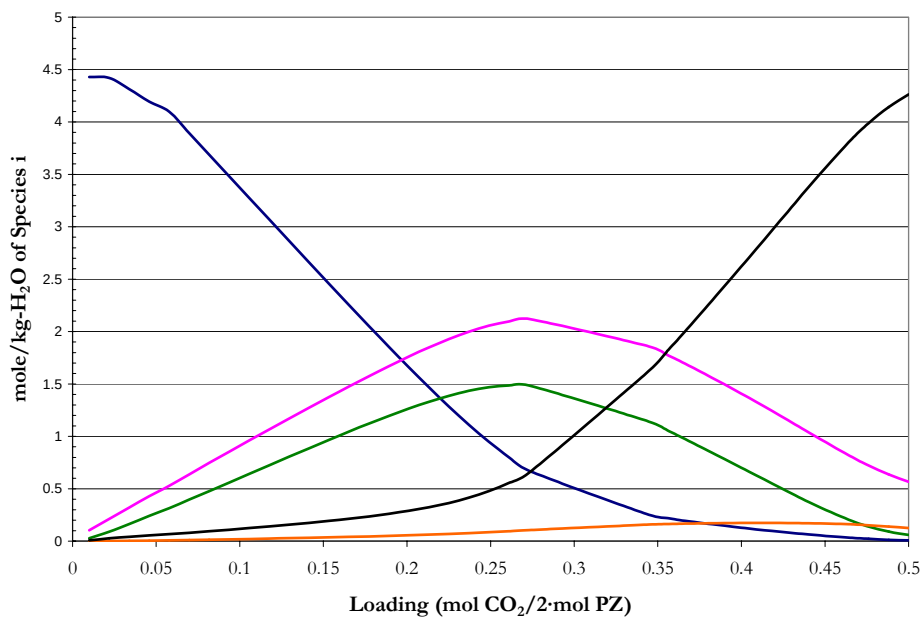
Figure 14.5-72. Predictions for the Liquid Phase Speciation in 5 m PZ at 40 °C from this work. Lines: —, PZ, —, PZH +1 , —, PZCOO -1 , —, PZ(COO -1 ) 2 , —, H + PZCOO -1 .
