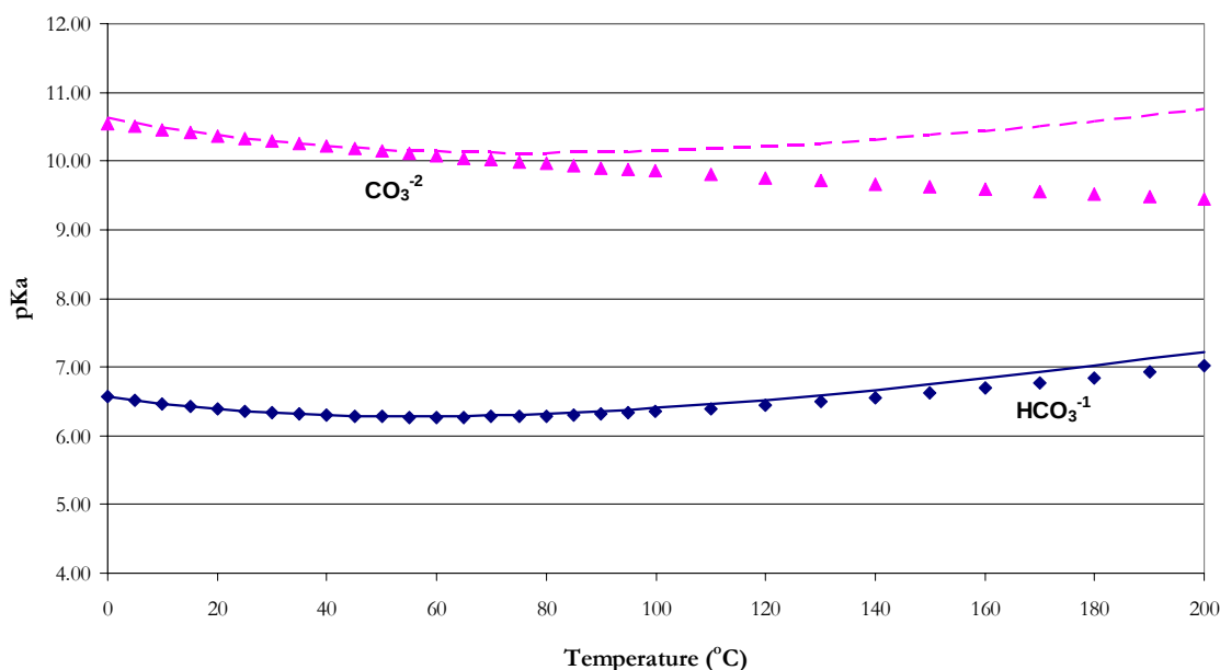
Figure 12.5-2. Comparison of the Dissociation Equilibrium Constant for \text{HCO}_3^{-1} and \text{CO}_3^{-2} (mole fraction based) from 0 – 200 °C. Points: \blacklozenge and \blacktriangle , Austgen et al. (1989). Lines: \text{—} , Edwards et al. (1978) based on Table 12.5-2.
