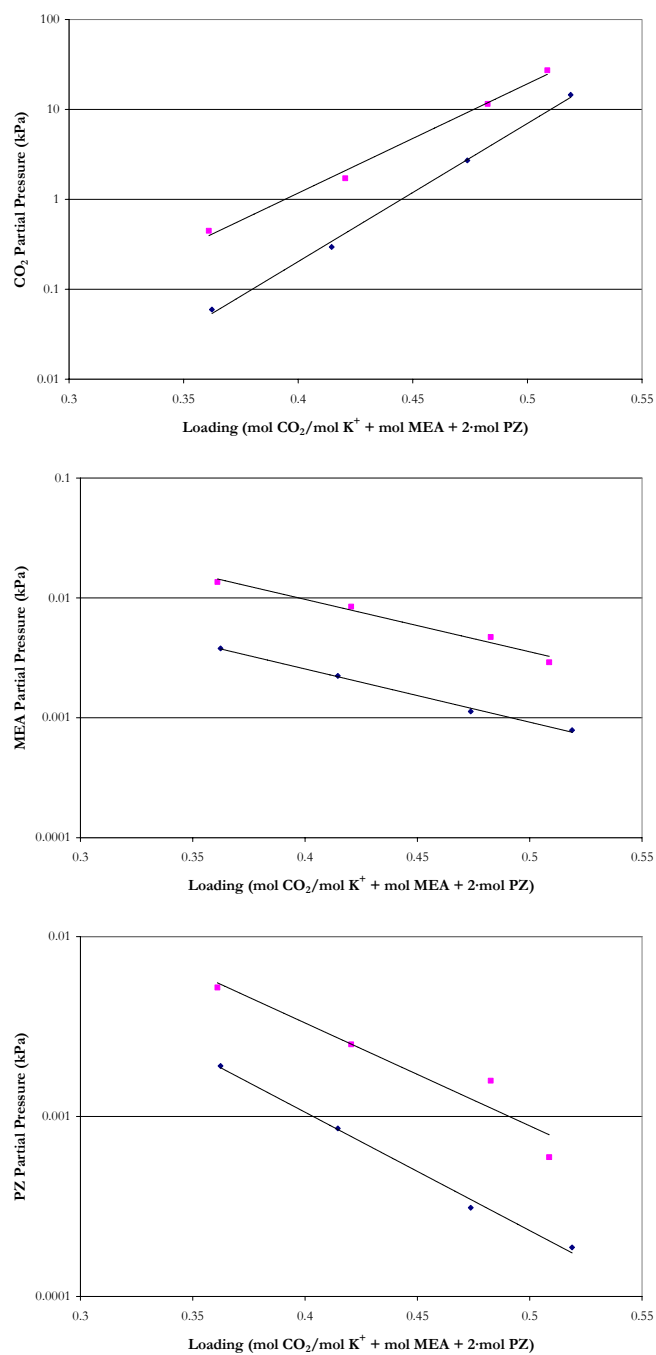
Figure 18.2-4. Experimental Data in Mixtures of 2.5 m K + + 7 m MEA + 2 m PZ at 40 and 60 °C from this work. Points: ◆ (40 °C) and ■ (60 °C). Lines: OLS Approximations.
