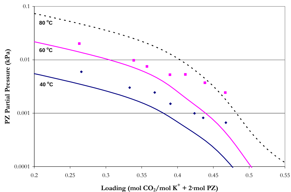
Figure 15.5-13. PZ Volatility in 3.6 m K + + 3.6 m PZ from 40 – 80 °C. Points: ♦, 40 °C and ■, 60 °C. Lines: elecNRTL Model Predictions.
