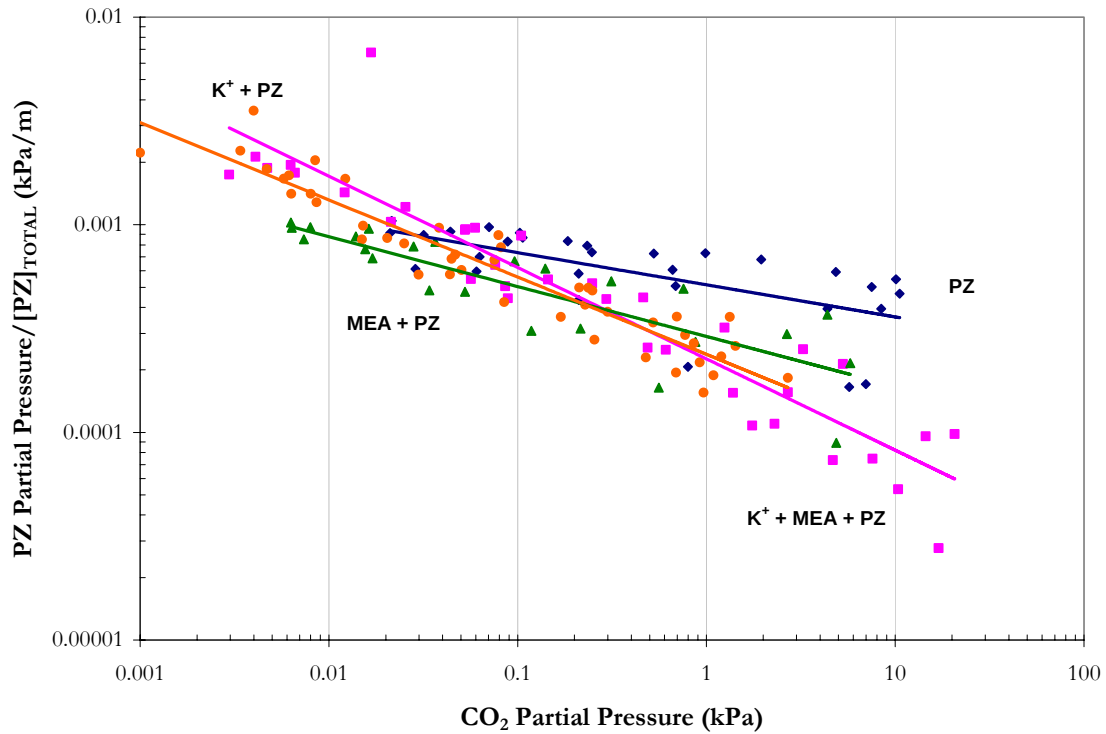
Figure 19.3-2. Comparison of Normalized PZ Volatility versus \text{CO}_2 Solubility at 40 °C from this work. Points: \blacklozenge , \text{H}_2\text{O} -PZ- \text{CO}_2 , \blacktriangle , \text{H}_2\text{O} -MEA-PZ- \text{CO}_2 , \bullet , \text{H}_2\text{O} - \text{K}_2\text{CO}_3 -PZ- \text{CO}_2 , \blacksquare , \text{H}_2\text{O} - \text{K}_2\text{CO}_3 -MEA-PZ- \text{CO}_2 . Lines: OLS Approximations.
