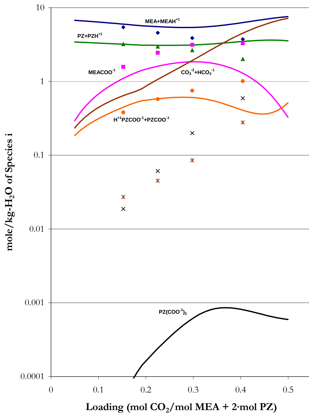
Figure 16.3-36. Liquid Phase Speciation from C 13 NMR in 7 m MEA + 3.6 m PZ at 60 °C. Points: ♦, MEA + MEAH + , ■, MEACOO - , ▲, PZ + PZH + , ●, H + PZCOO - + PZCOO - , ×, PZ(COO - ) 2 , *, CO 3 2- +HCO 3 - . Lines: elecNRTL Predictions.
