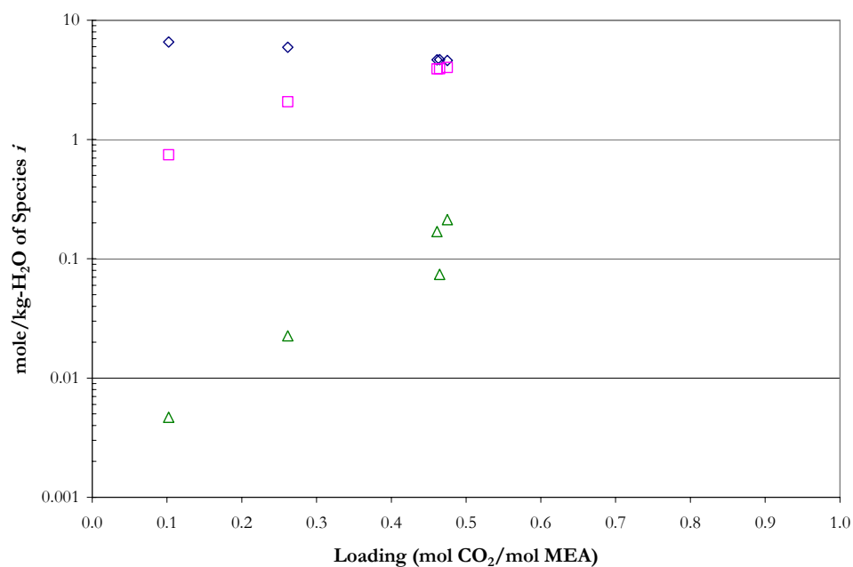
Figure 13.3-16. Liquid Phase Speciation from C 13 NMR at 60 °C. Points: ◇, MEA+MEA+H + , □, MEACOO - , △, CO 3 -2 +HCO 3 -1 , from this work.
