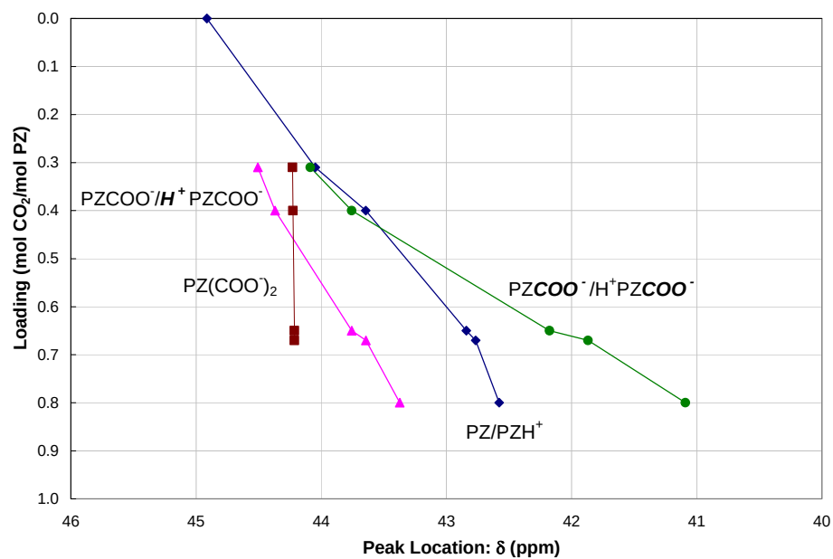
Figure 3.9-5. High Field 13 C Chemical Shifts for 2 m PZ at 27 °C with Varying CO 2 Loading.
