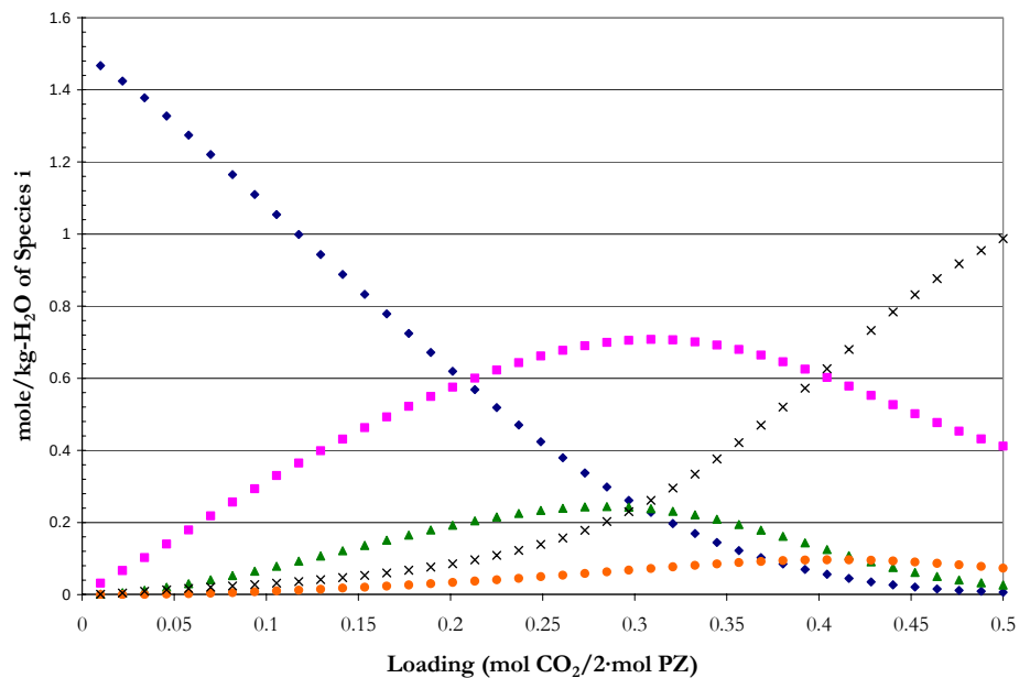
Figure 14.5-63. Predictions for the Liquid Phase Speciation in 1.5 m PZ at 40 °C from this work. Points: \blacklozenge , \text{PZ} , \blacksquare , \text{PZH}^{+1} , \blacktriangle , \text{PZCOO}^{-1} , \bullet , \text{PZ}(\text{COO}^{-1})_2 , \times , \text{H} + \text{PZCOO}^{-1} .
