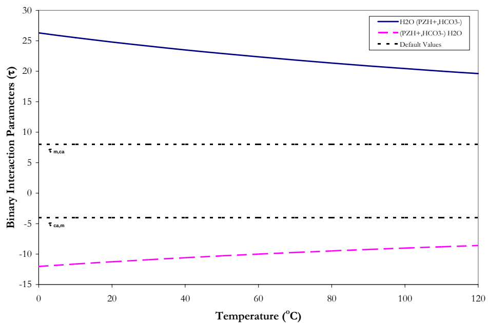
Figure 14.4-2. Binary Interaction Parameters for H 2 O, PZH + / HCO 3 - .
