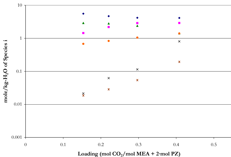
Figure 16.2-20. Liquid Phase Speciation from C 13 NMR at 27 °C. Points: ◆, MEA + MEAH + , ■, MEACOO - , ▲, PZ + PZH + , ●, H + PZCOO - + PZCOO - , ×, PZ(COO - ) 2 , *, CO 3 -2 +HCO 3 - .
