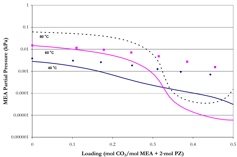
Figure 16.3-6. Experimental MEA Volatility in Mixtures of 3.5 m MEA Plus 3.6 m PZ at 40 and 60 °C from this work. Points: ♦ (40 °C) and ■ (60 °C). Lines: elecNRTL Predictions.
