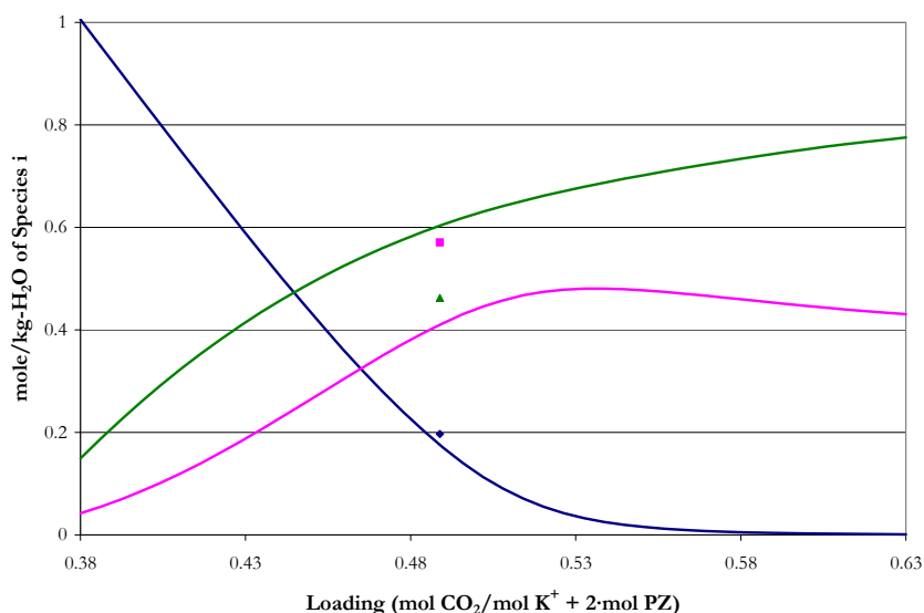
Figure 15.5-71. Comparison of Liquid Phase NMR Speciation in 6 m K^+ + 1.2 m PZ at 27 °C to Model Predictions. Points: \blacklozenge , PZ+PZH^{+1} , \blacksquare , PZCOO^{-1}+H^+PZCOO^{-1} , \blacktriangle , PZ(COO^{-1})_2 from Cullinane (2005). Lines: —, this work.
