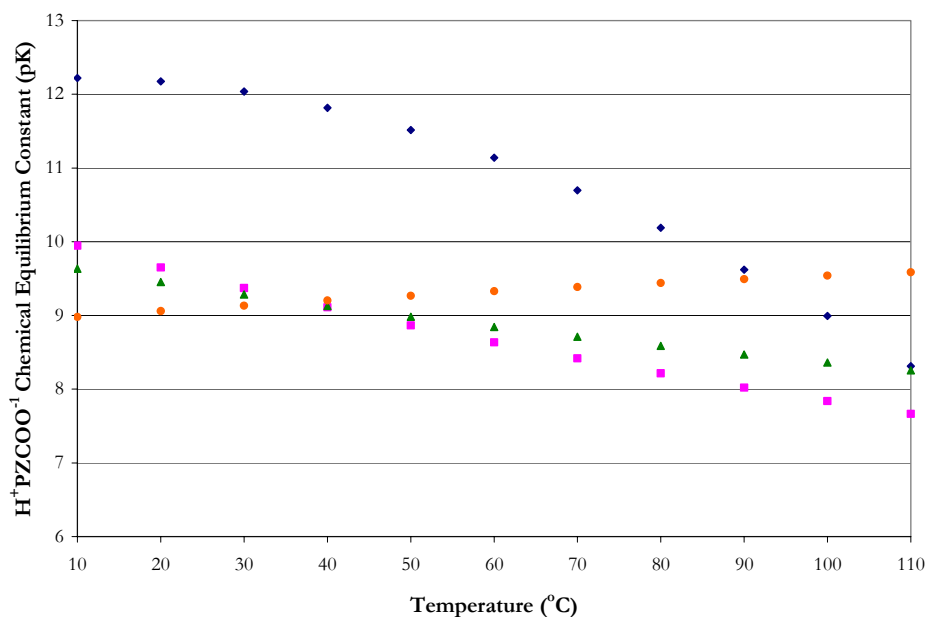
Figure 14.5-78. Comparison of the Chemical Equilibrium Constant of \text{H}^+\text{PZCOO}^- . Points: ●, Ermatchkov et al. (2003), ■, Cullinane (2005), ▲, Derks et al. (2005), ◆, this work.
