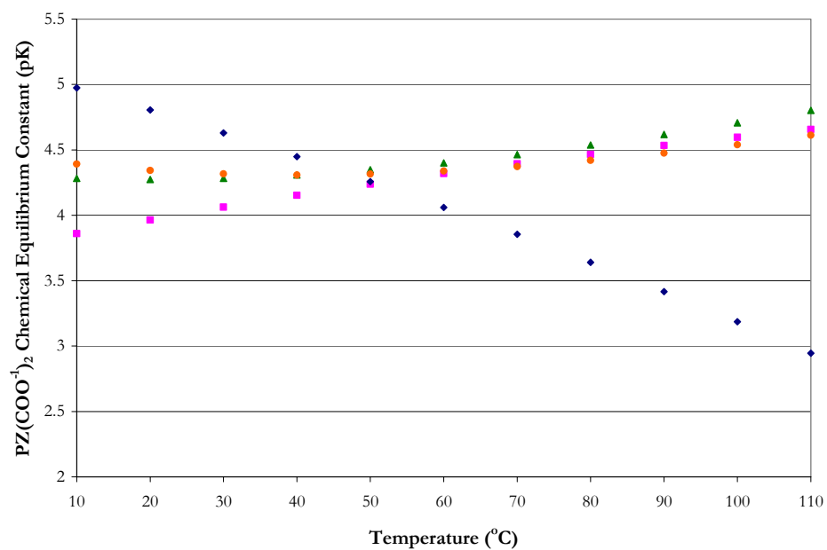
Figure 14.5-77. Comparison of the Chemical Equilibrium Constant of PZ(COO -1 ) 2 . Points: ●, Ermatchkov et al. (2003), ■, Cullinane (2005), ▲, Derks et al. (2005), ◆, this work.
