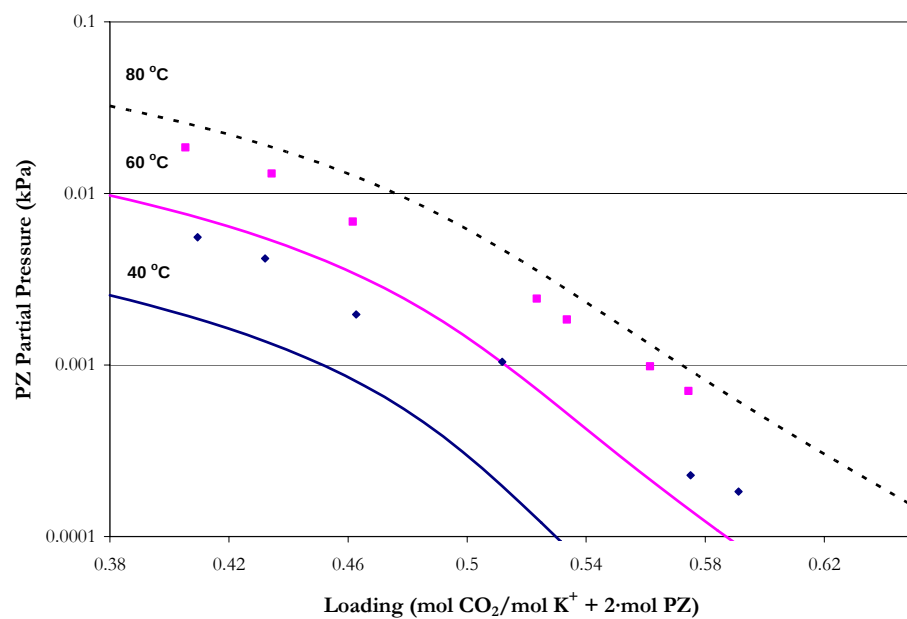
Figure 15.5-14. PZ Volatility in 6 m K + + 1.2 m PZ from 40 – 80 °C. Points: ♦, 40 °C and ■, 60 °C. Lines: elecNRTL Model Predictions.
