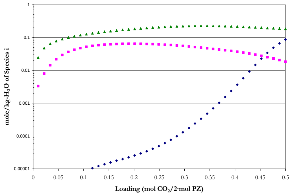
Figure 14.5-59. Predictions for the Liquid Phase Speciation in 1.5 m PZ at 25 °C from this work. Points: \blacklozenge , CO 2 , \blacksquare , CO 3 2- , \blacktriangle , HCO 3 - 1.
