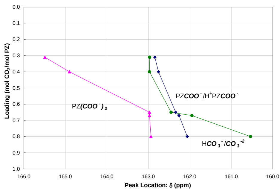
Figure 3.9-6. Low Field 13 C Chemical Shifts for 2 m PZ at 27 °C with Varying CO 2 Loading.
