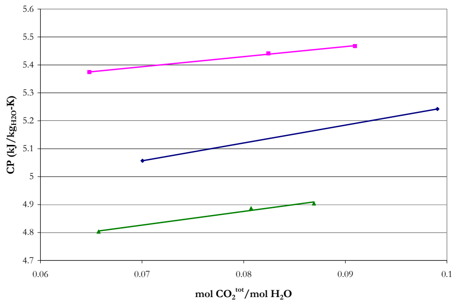
Figure 15.5-39. Apparent Partial Specific Heat Capacity for Mixtures of Potassium Carbonate + Piperazine at 80 °C. Points: \blacklozenge , 5 m K + + 2.5 m PZ, \blacksquare , 3.6 m K + + 3.6 m PZ, \blacktriangle , 6 m K + + 1.2 m PZ. Lines: OLS Approximations.
