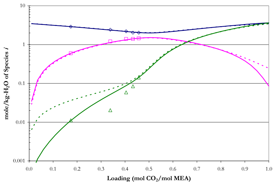
Figure 13.5-42. Comparison of Liquid Phase NMR Speciation in 3.5 m MEA at 27 °C to Model Predictions. Points: \diamond , MEA+MEA ^+ , \square , MEACOO ^{-1} , \triangle , CO _2 +CO _3^{-2} +HCO _3^{-1} , from this work. Lines: - - -, Austgen (1989), —, this work.
