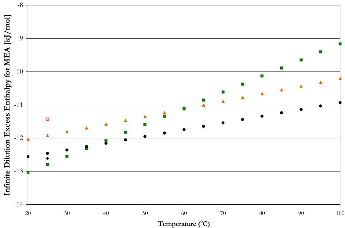
Figure 8.3-1. Infinite Dilution Excess Enthalpy for MEA from 20 to 100 °C. Points: ◆, Touhara et al. (1982), ◻, Kim et al. (1987), ▲, Austgen et al. (1991), ■, Posey (1996), and ●, this work.
