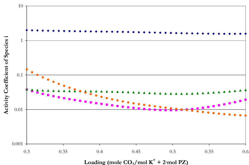
Figure 15.5-55. Predictions for the Liquid Phase Activity Coefficients in 5 m \text{K}^+ + 2.5 m PZ at 60 °C from this work. Points: \blacklozenge , \text{CO}_2 , \blacksquare , \text{CO}_3^{2-} , \blacktriangle , \text{HCO}_3^- , \bullet , \text{K}^+ .
