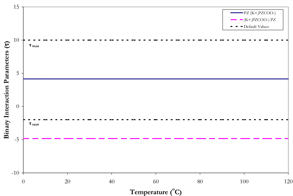
Figure 15.4-5. Binary Interaction Parameters for PZ, \text{K}^+/\text{PZCOO}^{-1} .
