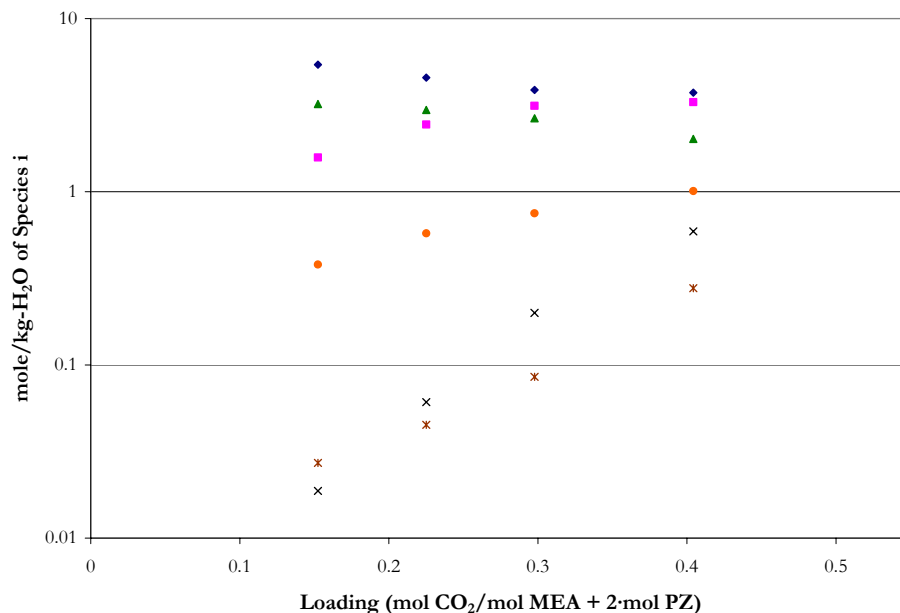
Figure 16.2-22. Liquid Phase Speciation from C 13 NMR at 60 °C. Points: ◆, MEA + MEAH + , ■, MEACOO - , ▲, PZ + PZH + , ●, H + PZCOO - + PZCOO - , ×, PZ(COO - ) 2 , *, CO 3 -2 +HCO 3 - .
