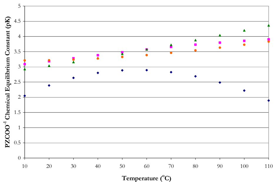
Figure 14.5-76. Comparison of the Chemical Equilibrium Constant of PZCOO -1 . Points: ●, Ermatchkov et al. (2003), ■, Cullinane (2005), ▲, Derks et al. (2005), ◆, this work.
