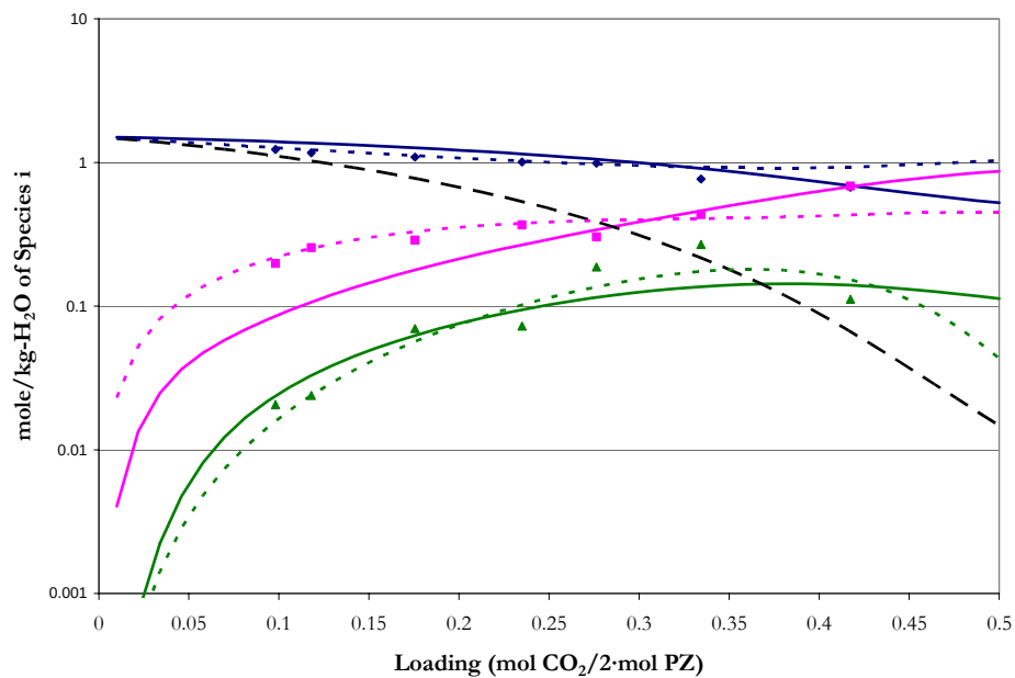
Figure 14.5-67. Comparison of Liquid Phase NMR Speciation in 1.5 m PZ at 60 °C to Model Predictions. Points: \blacklozenge , \text{PZ}+\text{PZH}^{+1} , \blacksquare , \text{PZCOO}^{-1}+\text{H}^+\text{PZCOO}^{-1} , \blacktriangle , \text{PZ}(\text{COO}^{-1})_2 from Ermatchkov et al. (2003). Lines: - - -, Hilliard (2005), —, this work, — —, Conc. Free PZ.
