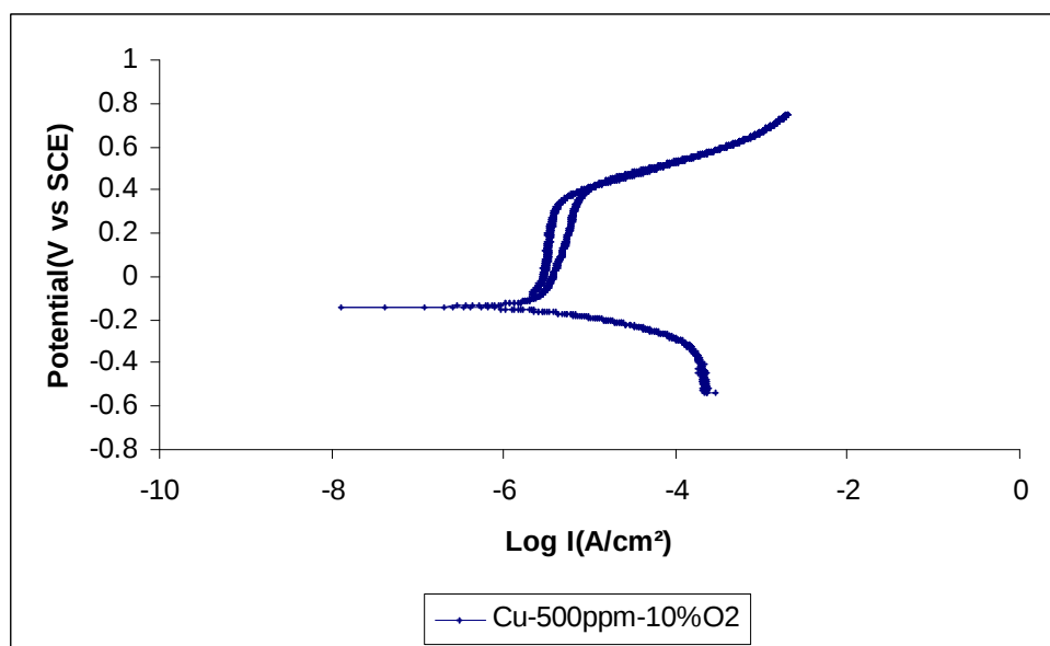
Figure 40: Cyclic polarization curve of carbon steel in 5 M MEA-1.2 M PZ containing 500 ppm \text{CuCO}_3 and 0.20 mol/mol \text{CO}_2 loading at 80°C with 10% oxygen.
