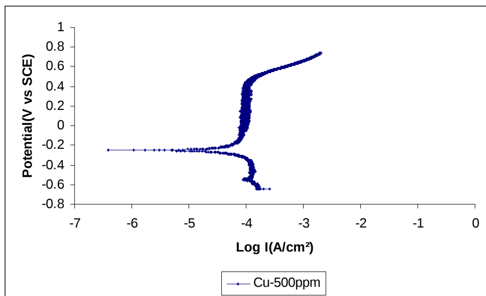
Figure 39: Cyclic polarization curve of carbon steel in 5 M MEA-1.2 M PZ containing 500 ppm \text{CuCO}_3 and 0.20 mol/mol \text{CO}_2 loading at 80°C
