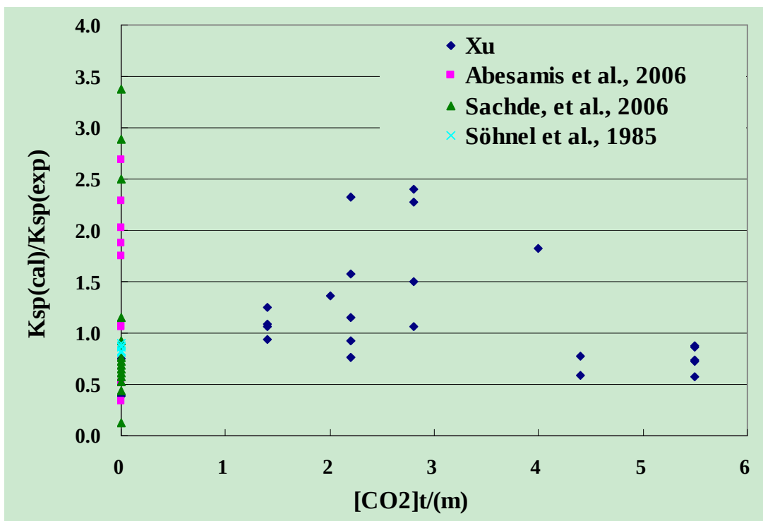
Figure 34: Accuracy of model 1 for \text{K}_2\text{SO}_4 solubility, effect of \text{CO}_2 loading
