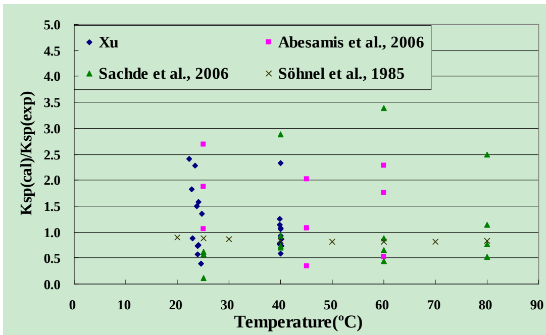
Figure 33: Accuracy of model 1 for \text{K}_2\text{SO}_4 solubility, effect of temperature
