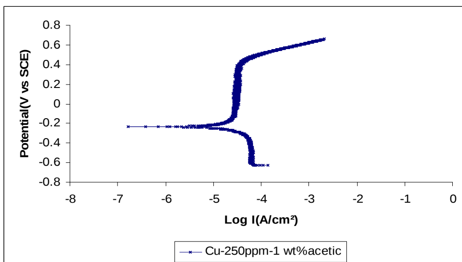
Figure 42: Cyclic polarization curve of carbon steel in 5 M MEA-1.2 M PZ containing 250 ppm \text{CuCO}_3 , 1 wt % acetic acid and 0.20 mol/mol \text{CO}_2 loading at 80^\circ\text{C}
