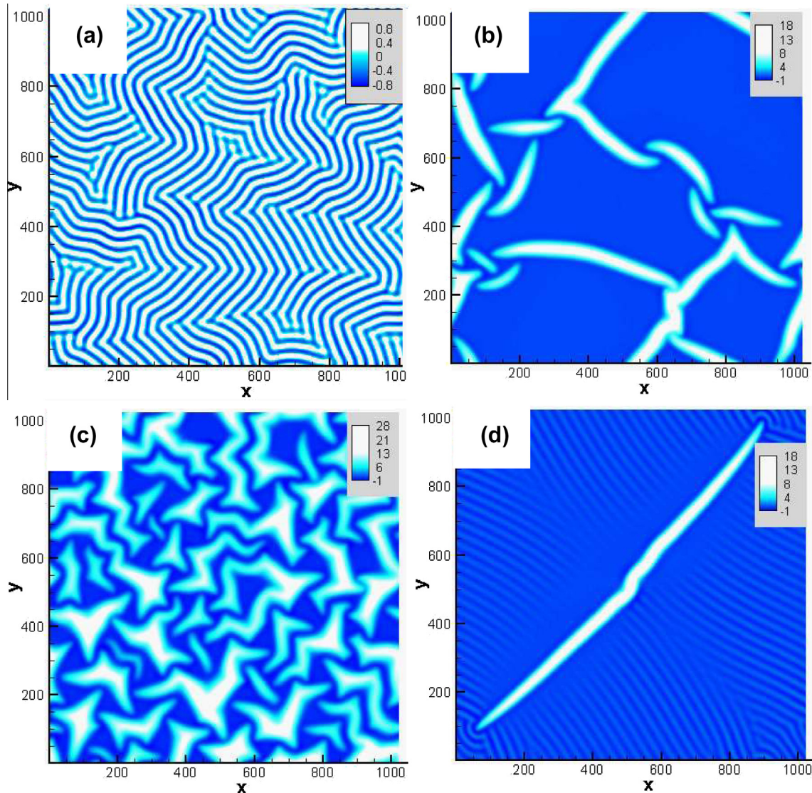
Fig. 11. Simulated post-buckling morphologies of the elastic film/substrate systems: (a)–(c) for increasing pre-strain, \epsilon_{pre} = 0.0095, 0.011 , and 0.04 , with \gamma_n/\gamma^* = 0.16 ; (d) for \epsilon_{pre} = 0.011 and \gamma_n/\gamma^* = 0.32 . In all cases, \mu_f/\mu_s = 420 and \gamma_t/\gamma_n = 10 .
