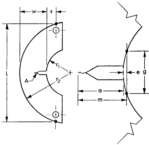
FIG. A6.2 Measurement of Outer Radius ( r_2 ) and Crack Size for the Arc-Shaped Tension A(T) Specimen (see A6.4.1)
