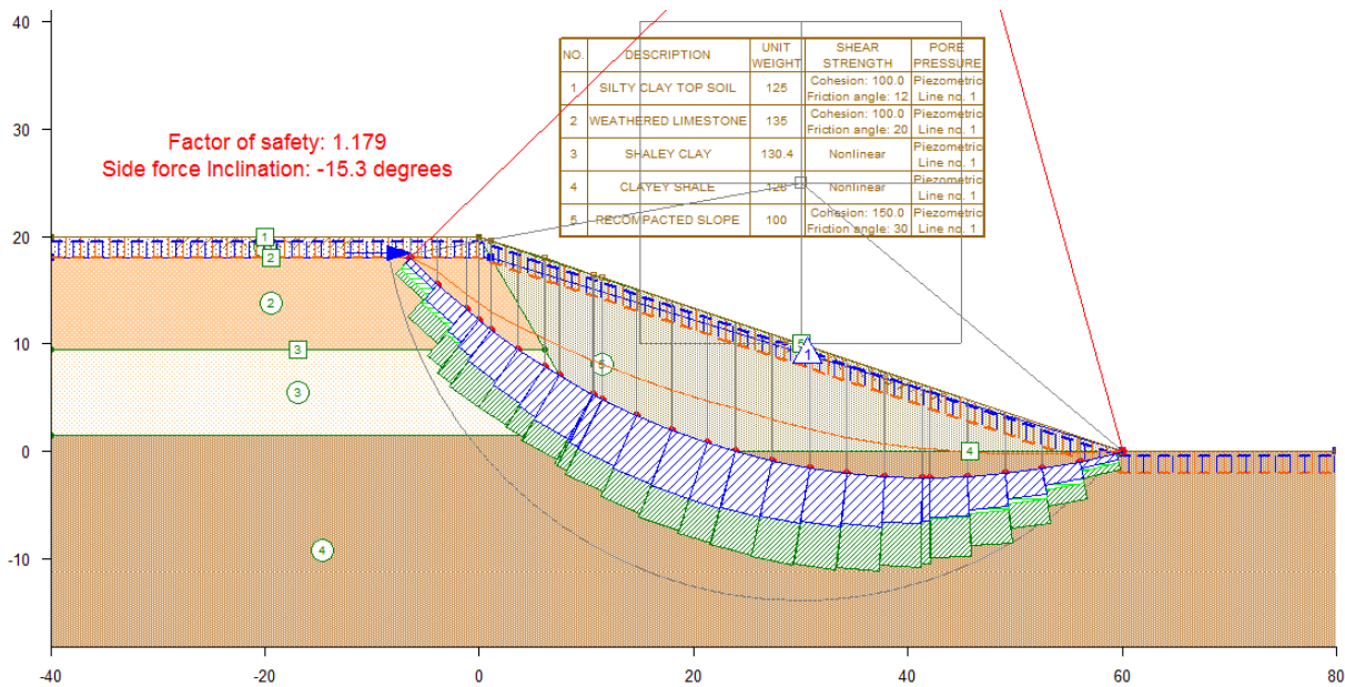
Figure 8.18: Limit Equilibrium Analysis of the Tire Shred Reinforced Re-Compacted Soil Embankment
