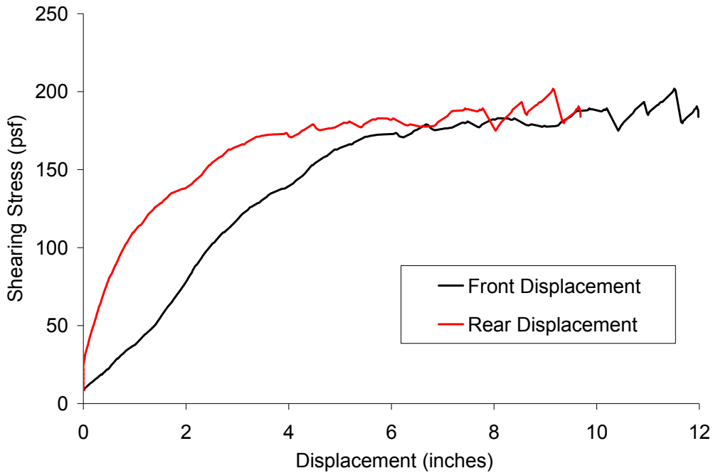
Figure 6.8: Interface Shearing Stress versus Tire Bale Displacement for the Dry Tire Bale Interface
