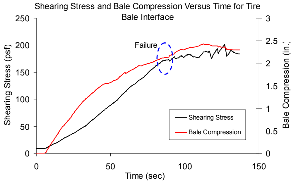
Figure D.30: Interface Shearing Resistance and Tire Bale Compression versus Elapsed Testing Time for the Dry Tire Bale Only Interface (Normal Stress = 180 psf)
