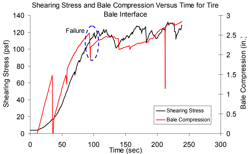
Figure E.13: Interface Shearing Resistance and Tire Bale Compression versus Elapsed Testing Time for the Wet Anisotropic Tire Bale Only Interface (Normal Stress = 216 psf)
