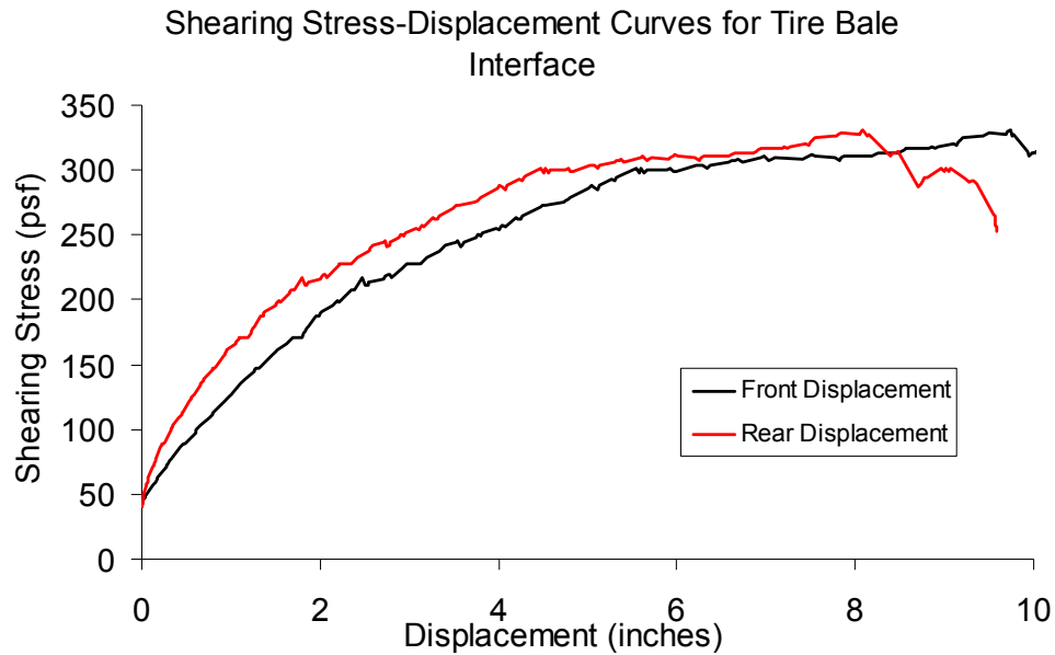
Figure D.48: Interface Shearing Resistance versus Displacement for the Dry Tire Bale Only Interface (Normal Stress = 361 psf)
