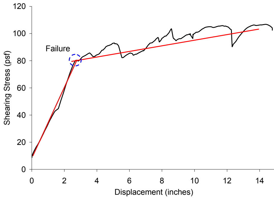
Figure 6.15: Illustration of the Bi-Linear Method to Determine Peak Interface Strength
