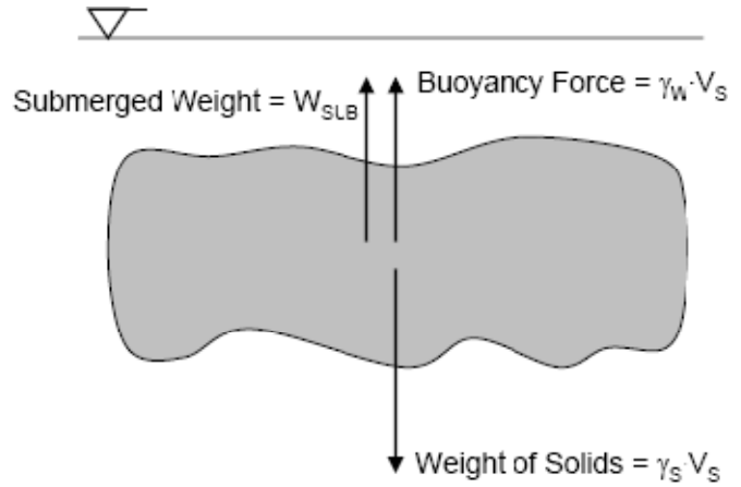
(b) Forces Acting on Submerged Bale.
