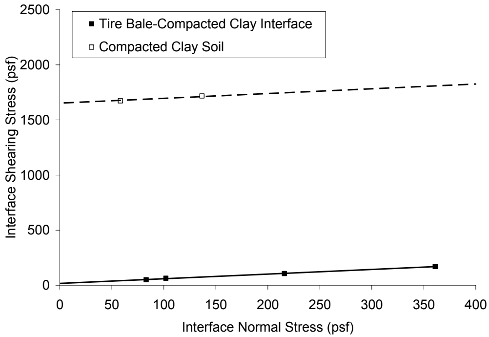
Figure 6.32: Comparison of the Clay Strength from Undrained Direct Shear and the Tire Bale-Clay Interface Testing
