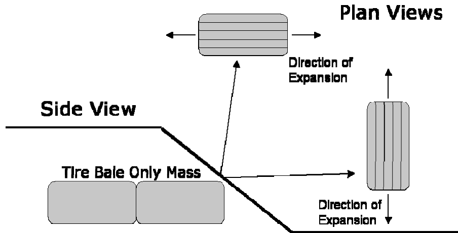
Figure 6.24: Illustration of Traditional and Anisotropic Tire Bale Placement in a Tire Bale Only Slope
