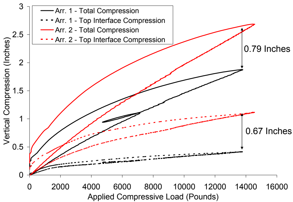
Figure 7.10: Total Compression and Top Interface Compression Curves for the Two Bale Arrangements for the Three Bale Structures
