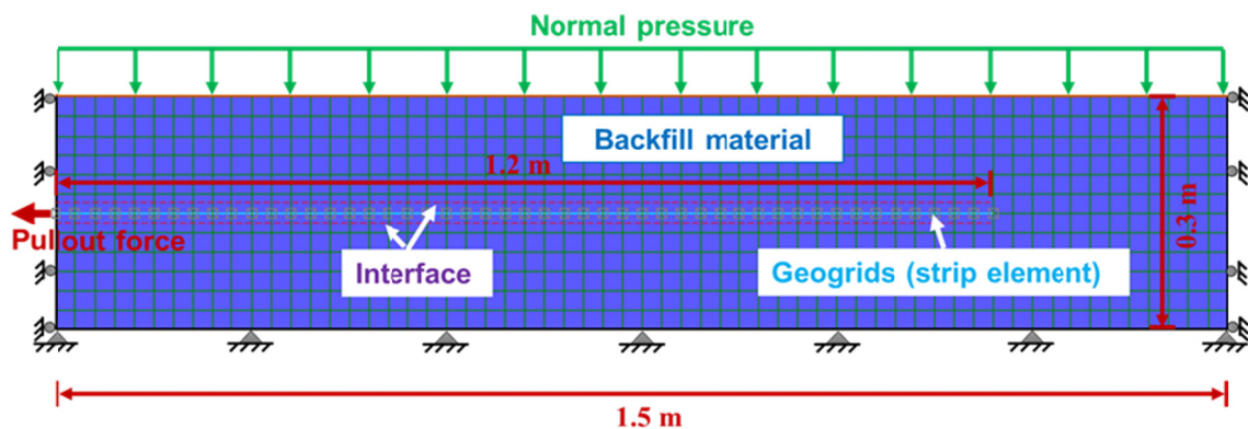
Figure 1. Mesh of numerical model
