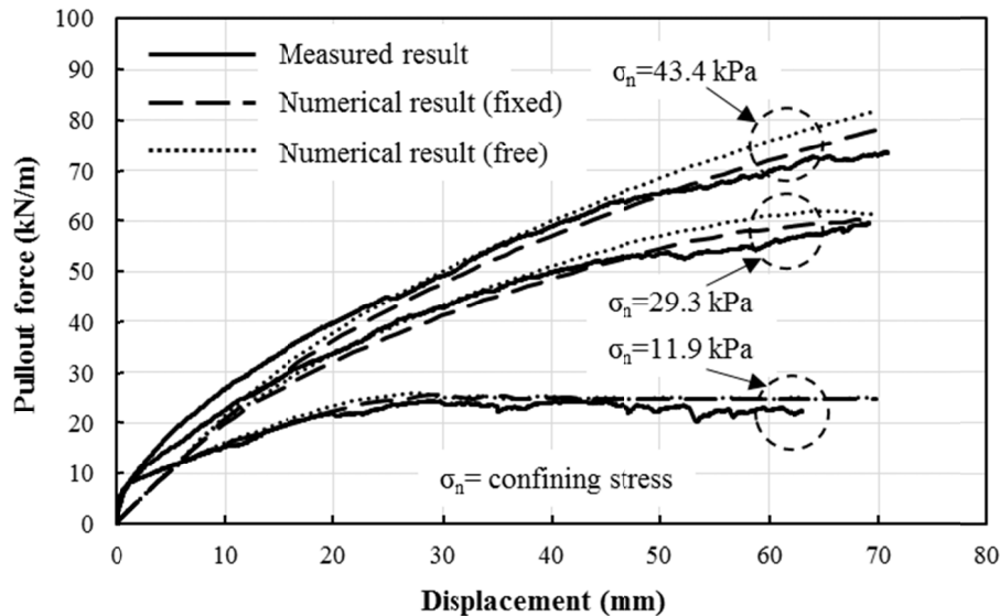
Figure 3. Comparison between measured and numerically calculated pullout test results
