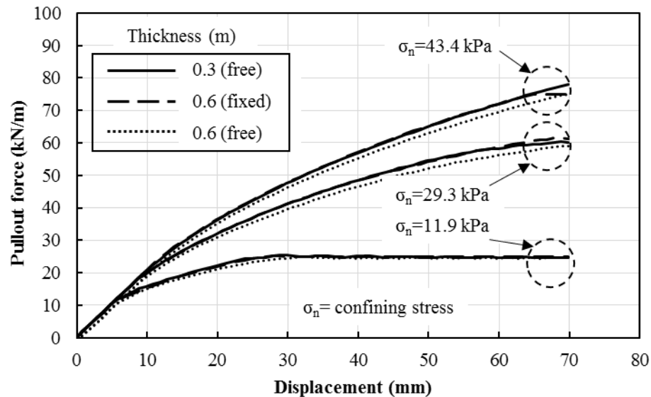
Figure 4. Influence of backfill thickness
