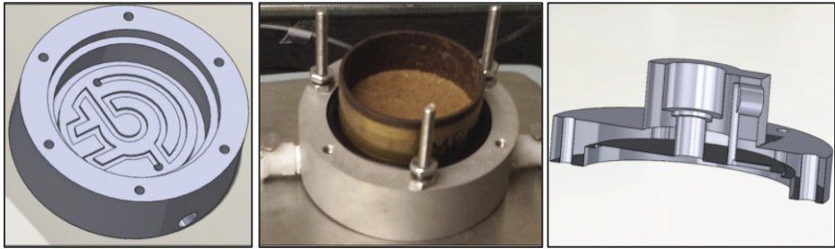
Figure 1. Base detail: a) 3D view of base design, b) sample mounted in the base, c) cross section of the cap
