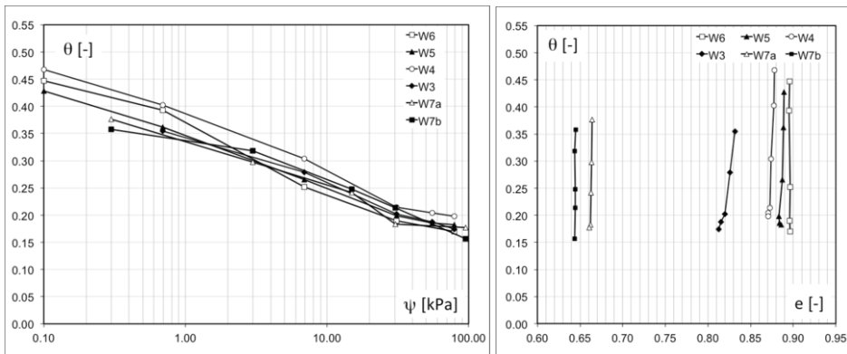
Figure 4. (a) Soil-water retention curve ( \theta - \psi ), (b) \theta - e relationship.
