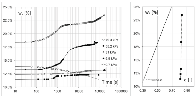
Figure 6. (a) Evolution of gravimetric water content with time, (b) relationship between water content and void ratio at the end of each stage.
