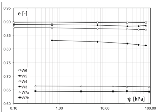
Figure 5. Changes in void ratio with suction ( e - \psi ).
