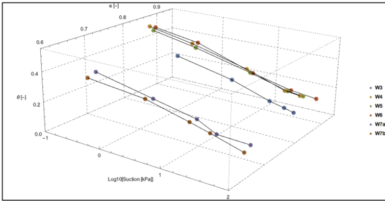
Figure 3. Multiple stages on wetting hydro-mechanical path.
