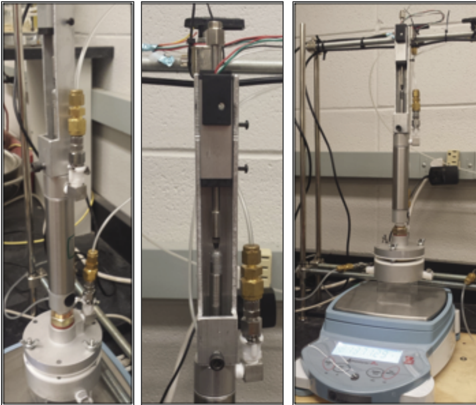
Figure 2. View of the piston and air connections (a); detail of the bracket and LVDT (b); and complete chamber mounted over the scale (c).
