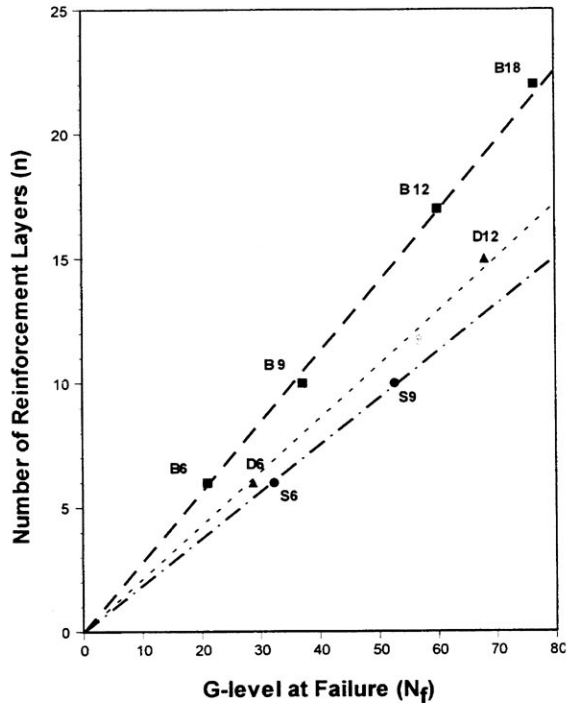
Figure 7 - G-level at failure for the centrifuge models
