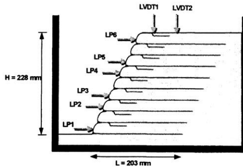
Figure 1 - Typical centrifuge model
