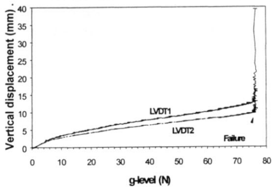
Figure 4 - Settlements at the crest of a reinforced slope model
