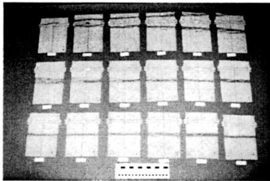
Figure 6 - Geotextile reinforcements retrieved after testing
