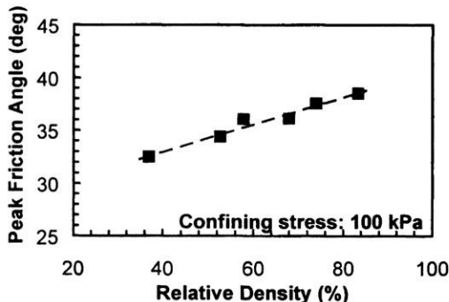
Figure 2 - Friction angle for Monterey No. 30 sand obtained from triaxial testing at different relative densities.
