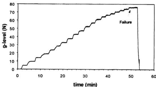
Figure 3 - G-level (N) versus time during centrifuge testing
