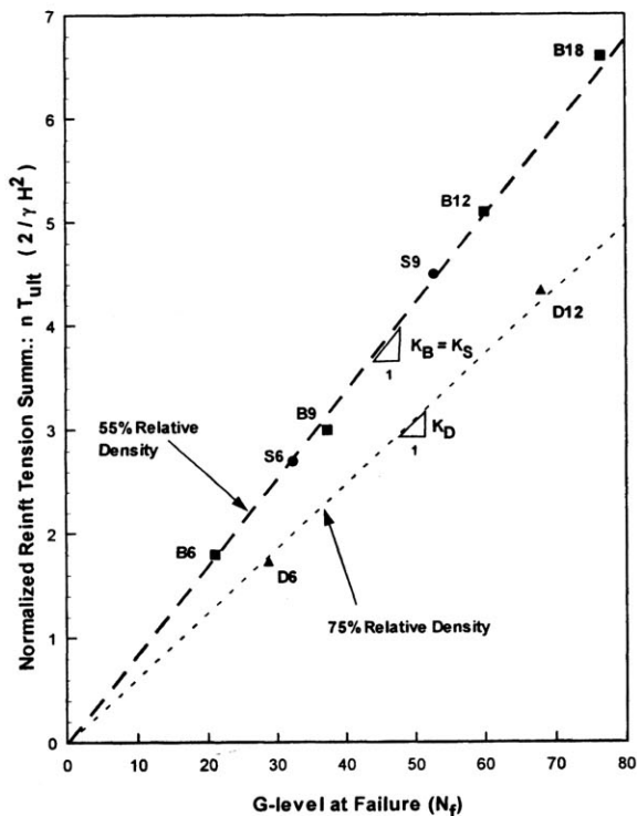
Figure 8 - Normalized Reinforcement Tension Summation (RTS) values from centrifuge test results
