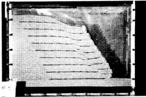
Figure 5 - Failed geotextile-reinforced slope model
