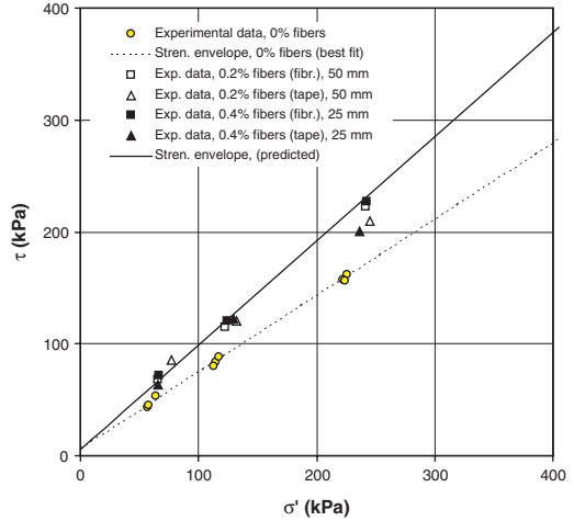
Figure 24. Consolidated shear strength results for specimen reinforced with 50 mm-long fibers (1000 denier) placed at \chi_w = 0.2\% and 25 mm fibers placed at \chi_w = 0.4\% , Soil 1.
