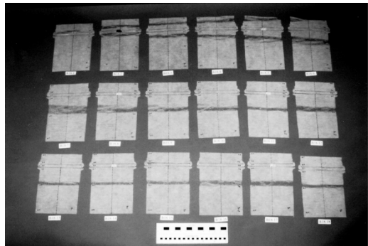
Figure 7. Geotextile reinforcements retrieved after testing.
