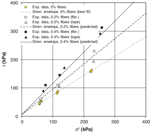
Figure 20. Comparison between predicted and experimental shear strength results for specimens reinforced at \chi_w = 0, 0.2\%, 0.4\% with 25 mm-long fibers (360 denier), Soil 1.
