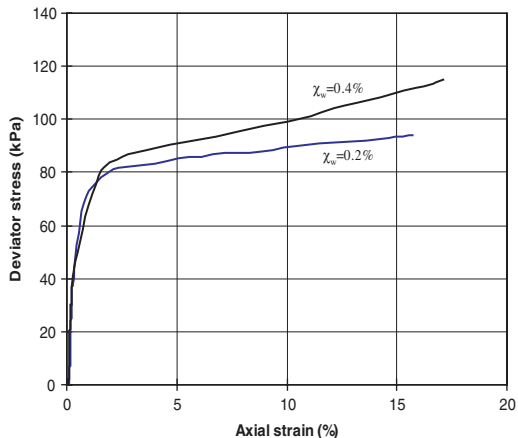
Figure 18. Stress-strain behavior of specimens prepared using \chi_w = 0.2, 0.4\% , with l_f = 25 mm fibers (2610 denier), \sigma_3 = 116 kPa, Soil 2.
