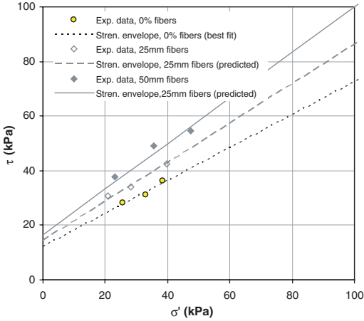
Figure 23. Comparison between predicted and experimental shear strength results for specimens reinforced with \chi_w = 0.4\% , with 25 mm-long and 50 mm-long fibers (2610 denier), Soil 2.
