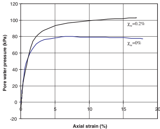
Figure 17. Excess pore water pressure of specimens prepared using \chi_w = 0, 0.2\% , with l_f = 50 mm fibers (2610 denier), \sigma_3 = 98 kPa, Soil 2.
