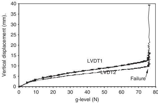
Figure 5. Settlements at the crest of a reinforced slope model.
