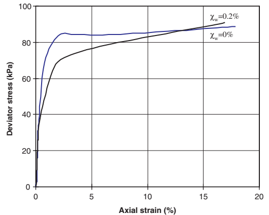
Figure 16. Stress-strain behavior of specimens prepared using \chi_w = 0, 0.2\% , with l_f = 50 mm fibers (2610 denier), \sigma_3 = 98 kPa, Soil 2.
