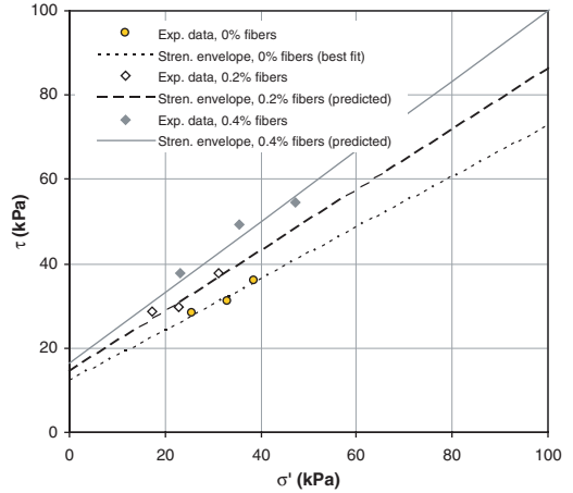
Figure 21. Comparison between predicted and experimental shear strength results for specimens reinforced at \chi_w = 0, 0.2\%, 0.4\% with 50 mm-long fibers (2610 denier), Soil 2.
