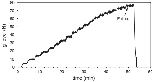
Figure 4. G-level (N) versus time during centrifuge testing.
