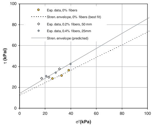
Figure 25. Consolidated shear strength results for specimen reinforced with 50 mm-long fibers (2610 denier) placed at \chi_w = 0.2\% and 25 mm fibers placed at \chi_w = 0.4\% , Soil 2.
