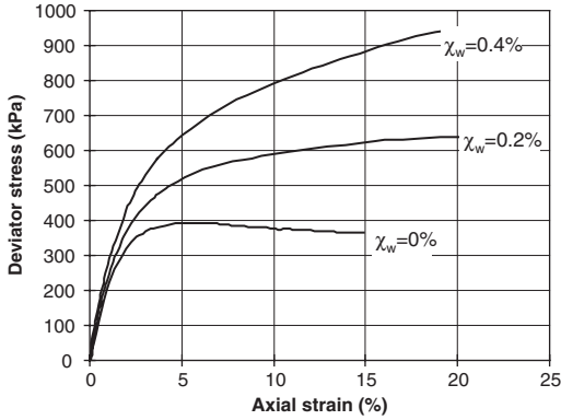
Figure 13. Stress-strain behavior of specimens prepared using \chi_w = 0, 0.2 and 0.4\% with l_f = 25 mm fibers (360 denier), \sigma_3 = 140 kPa, Soil 1.
