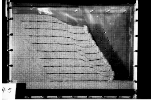
Figure 6. Failed geotextile-reinforced slope model.
