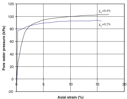
Figure 19. Excess pore water pressure of specimens prepared using \chi_w = 0.2, 0.4\% , with l_f = 25 mm fibers (2610 denier), \sigma_3 = 116 kPa, Soil 2.
