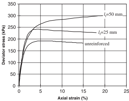
Figure 14. Stress-strain behavior of specimen prepared using \chi_w = 0.2\% , with l_f = 25 mm and 50 mm fibers (1000 denier), \sigma_3 = 70 kPa, Soil 1.
