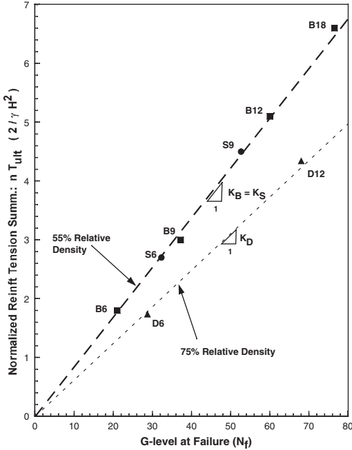
Figure 9. Normalized Reinforcement Tension Summation (RTS) values from centrifuge test results.
