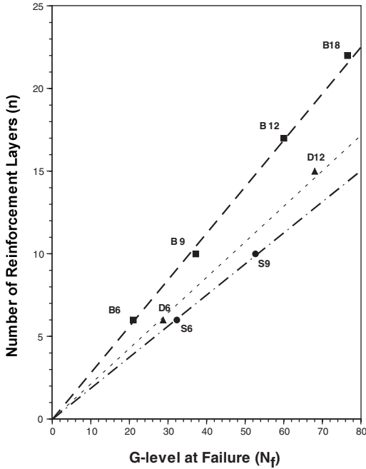
Figure 8. G-level at failure for the centrifuge models.
