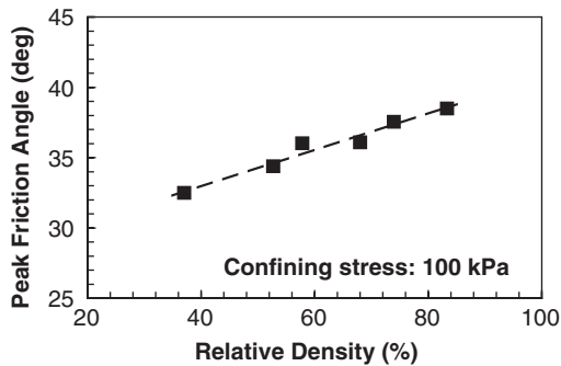
Figure 3. Friction angle for Monterey No. 30 sand obtained from triaxial testing at different relative densities.
