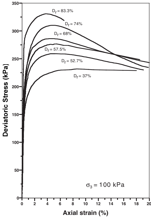
Figure 2. Stress strain behavior of Monterey No. 30 sand pluviated at different relative densities and tested in triaxial compression under the same confinement.
