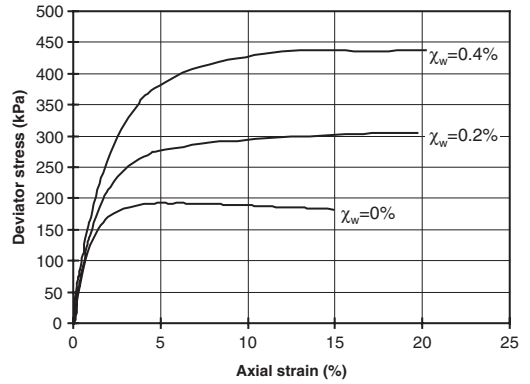
Figure 12. Stress-strain behavior of specimens prepared using \chi_w = 0, 0.2 and 0.4\% with l_f = 25 mm fibers (360 denier), \sigma_3 = 70 kPa, Soil 1.
