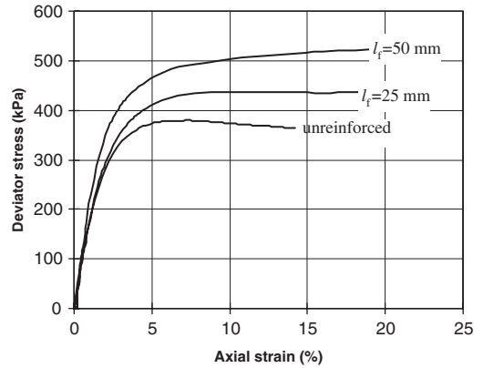
Figure 15. Stress-strain behavior of specimen prepared using \chi_w = 0.2\% , with l_f = 25 mm and 50 mm fibers (1000 denier), \sigma_3 = 140 kPa, Soil 1.
