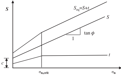
Figure 11. Representation of the equivalent shear strength according to the discrete approach.
