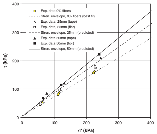
Figure 22. Comparison between predicted and experimental shear strength results for specimens reinforced at \chi_w = 0.2\% , with 25 mm-long and 50 mm-long fibers (1000 denier), Soil 1.
