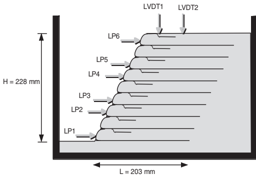
Figure 1. Typical centrifuge model.
