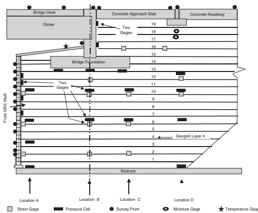
Figure 10. Instrumentation plan of Phase II structure.
