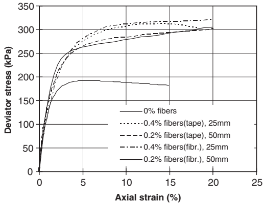
Figure 26. Comparison between stress-strain behavior for specimen reinforced with 50 mm fibers (1000 denier) placed at \chi_w = 0.2\% and 25 mm fibers placed at \chi_w = 0.4\% , \sigma_3 = 70 kPa.
