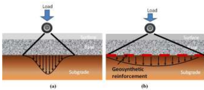
Figure 2: Relative load magnitudes at subgrade layer level for (a) unreinforced flexible pavement and (b) geosynthetic-reinforced flexible pavement
