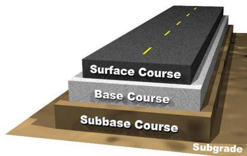
Figure 1: Cross-section of flexible pavement system (Muench 2006)
