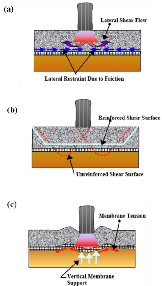
Figure 3: Reinforcement mechanisms induced by geosynthetics (Holtz et al. 1998): (a) Lateral restraint; (b) Increased bearing capacity; and (c) Membrane support
