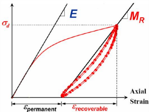
Figure 5: Comparison of Resilient Modulus, M_R , and Modulus of Elasticity, E
