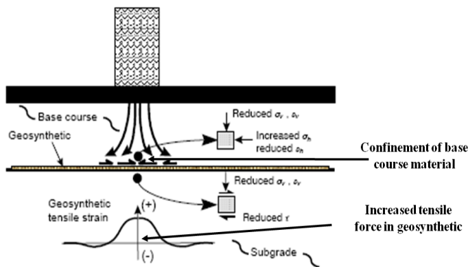
Figure 7: Mechanisms due to soil-geosynthetic interaction in geosynthetic-reinforced pavement that have been tried to be represented in laboratory tests (Perkins 1999)
