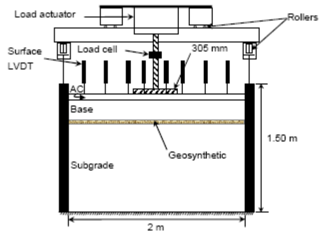
Figure 9: Cyclic plate load test (Perkins 1999)
