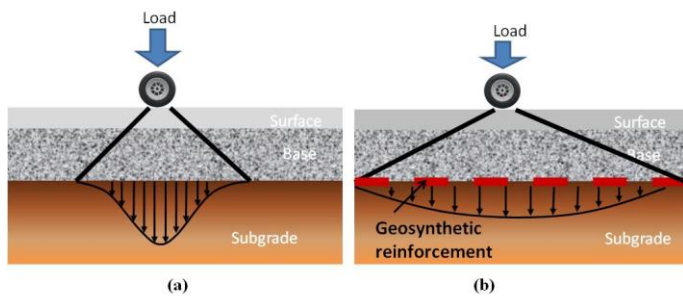
Figure 2: Relative load magnitudes at subgrade layer level for (a) unreinforced flexible pavement and (b) geosynthetic-reinforced flexible pavement
