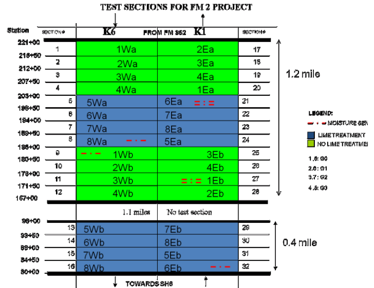
Figure 6: Schematic layout of test sections at FM 2 site
