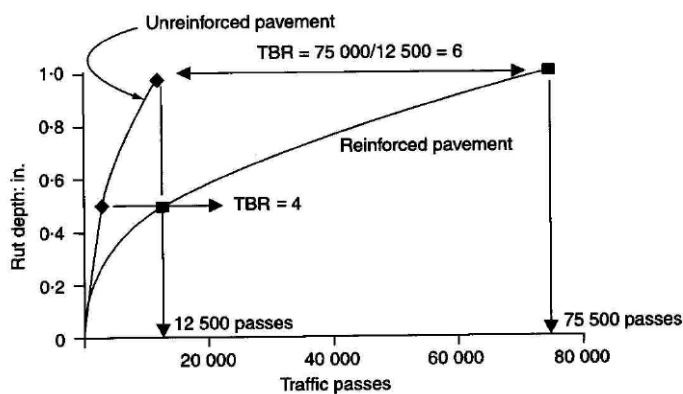
Figure 4: Typical TBR values for an unreinforced and reinforced pavement to reach a given rutting depth (Shukla 2002)
