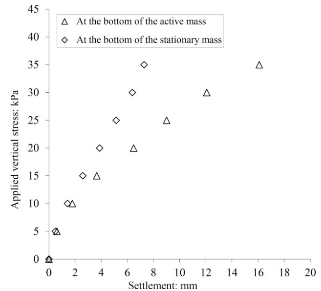
Figure 14. Applied vertical stress at load plate plotted against settlements measured at bottom of yielding and stationary masses
