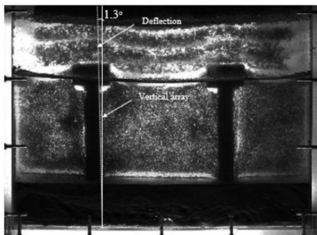
Figure 16. Image of pile deflection
